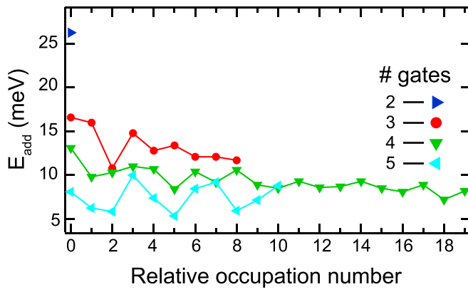
FIG. 3. Extracted values of E_{add} for various QD lengths as a function of relative occupation number.
