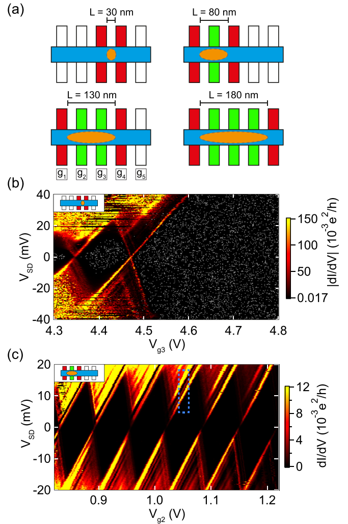
FIG. 2. (a) Schematic picture of the gate configurations used to form QDs (orange) of different lengths using 2, 3, 4, and 5 gates, respectively. (b) Lock-in signal dI/dV versus V_{SD} and V_{g3} of QD formed by two gates. To enhance contrast, values below the colorscale were given a grey color. Here, V_{g4} = 1700 mV. (c) Lock-in signal dI/dV versus V_{SD} and V_{g2} of QD formed by three gates. Here, V_{g1} = 2000 mV and V_{g3} = 4000 mV. Blue dashed rectangle shows an example of an averaging window used to extract excited state energies. Insets in (b) and (c) schematically show used gate configurations.
