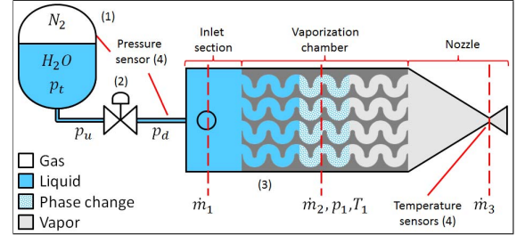
Fig. 1. VLM system showing: 1) a tank; 2) a valve; 3) a thruster, and 4) sensors. The mass flow rate \dot{m}_1 is the liquid flow rate, \dot{m}_2 is the vaporization rate, and \dot{m}_3 is the mass flow of the nozzle.
