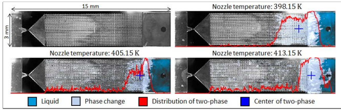
Fig. 4. Snapshots used for the measurement of the volume. An empty thruster is shown on the top-left corner for reference.
