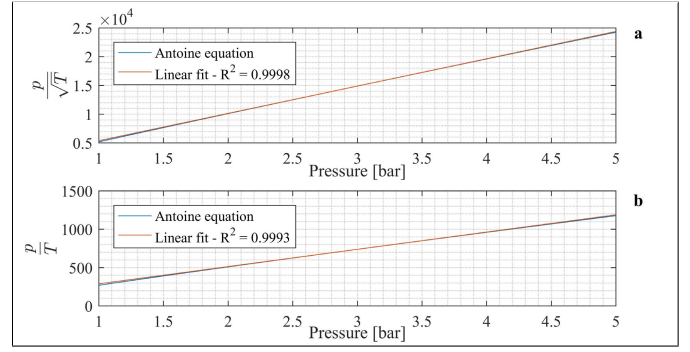
Fig. 3. Linear approximation of the pressure and temperature terms used in the modeling considering 401 points calculated using (11).
