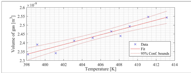
Fig. 5. Linear fitting of the volume of vapor inside the chamber as a function of the nozzle temperature for a pressure of 5 bar.
