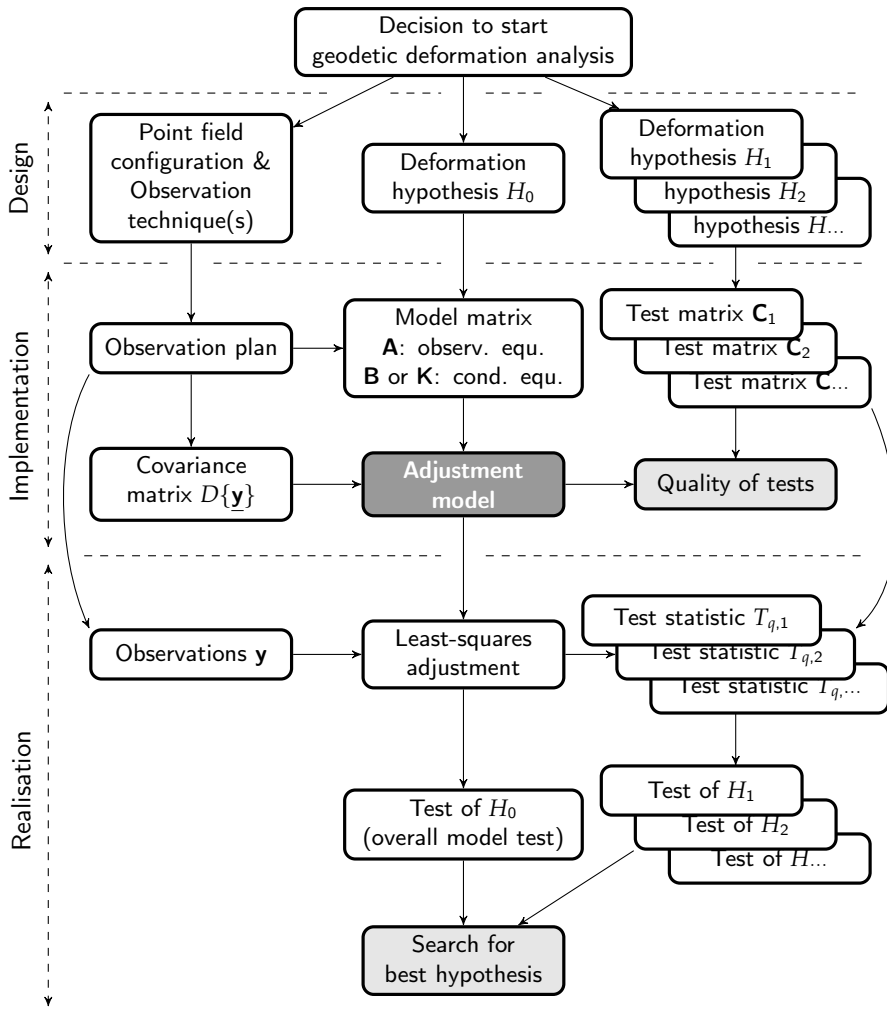
Figure 2.1: Analysis model: Geodetic deformation analysis, divided in three stages: design, implementation and realisation. \underline{y} , D\{\underline{y}\} , \underline{A} , \underline{B} , \underline{C}_1 , etc.: variable names used in this study.
