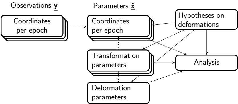
Figure 2.3: Coordinates model: adjustment in two phases. Dotted lines link elements that constitute the parameter vector. Arrows mean “determine(s), are (is) the basis for”. \underline{y} , \hat{\underline{x}} : variable names used in this study.
