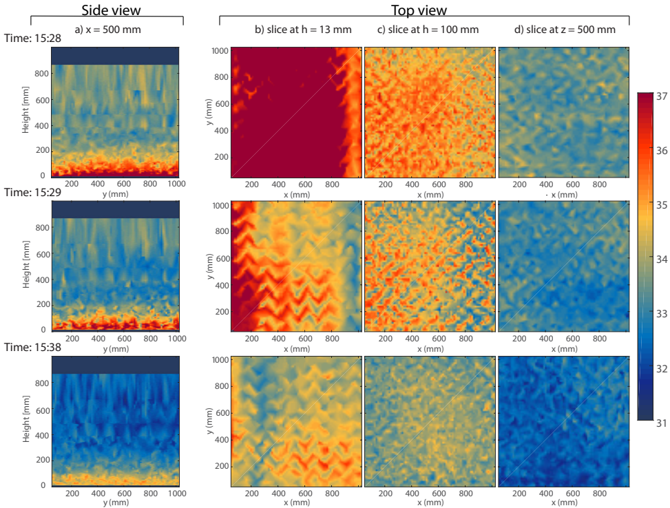
Figure 5.6: Vertical and horizontal profiles for the fourth experiment measured right before the uchimizu (15:28), right after (15:29), and 9 minutes after (15:38). Subplots in column a) show vertical cross-sections through the middle of the setup ( x = 500 mm), and subplots in columns b), c), and d) show horizontal cross-sections at height h = 13 mm, h = 100 mm, and h = 500 mm, respectively.
