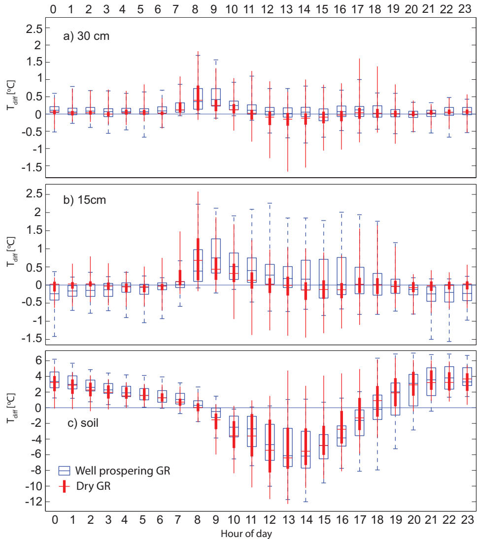
Figure II: Averages for each hour of a day for temperature difference ( T_{GR7} - T_{WG} ) 30 cm above the roof surface (a), 15 cm above the roof surface (b) and in the soil (c) for well prospering green roof (blue boxes, 2013) and dried out green roof (red bars, 2012). On each box or bar, the central mark is the median, and the edges of the box or the spread of the bar are the 25th and 75th percentiles. Whiskers represent extreme values excluding outliers.
