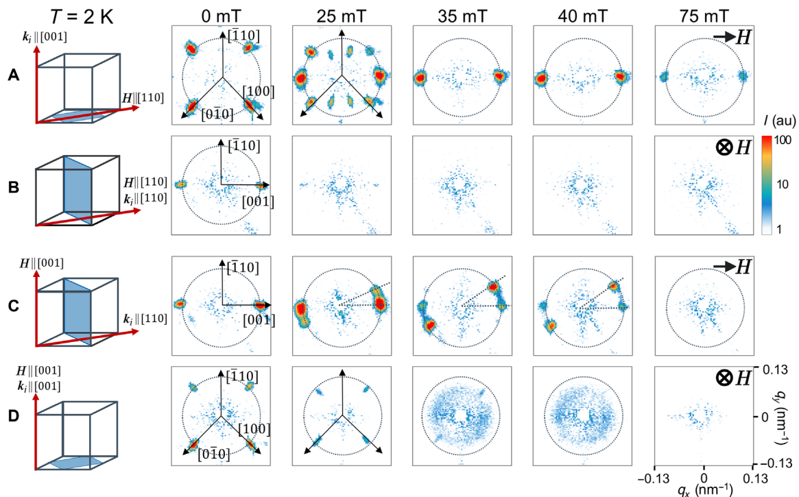
Fig. 1. Magnetic field dependence of the \text{Cu}_2\text{OSeO}_3 SANS patterns at T = 2 K. The first column illustrates the geometry of the experiment: H \parallel [110] in (A) and (B) and H \parallel [001] in (C) and (D). The orientation of the neutron beam wave vector is k_i \perp H in (A) and (C) and k_i \parallel H in (B) and (D). The blue planes illustrate the SANS detection plane. The radius of the dashed circles on the SANS patterns corresponds to the modulus of the helical spiral propagation vector Q = 2\pi/\ell \sim 0.1 \text{ nm}^{-1} , with \ell \sim 60 \text{ nm} being the pitch of the helix. au, arbitrary units.
