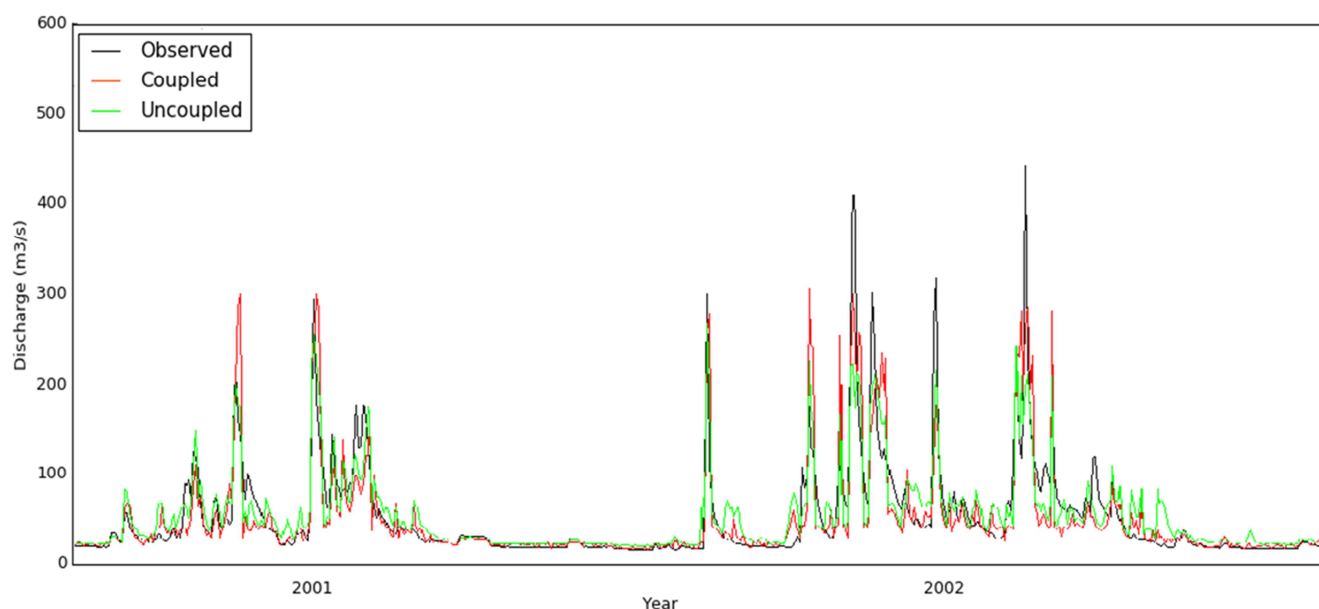
Figure 7. A closer look of the coupled and uncoupled flow simulations (2001-2002)
