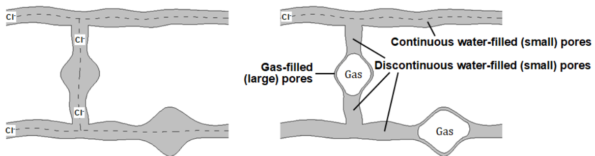
Fig. 3.11 Transport of chloride ions ( \text{Cl}^- ) in saturated (left) and non-saturated (right) pore systems.
