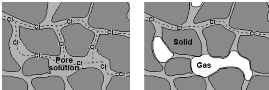
Fig. 2.3 Transport of chloride ions ( Cl^- ) in saturated (left) and unsaturated (right) porous systems.
