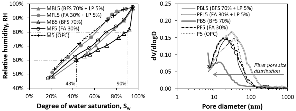
Fig. 6.13 (left) RH- S_w relations in blended mortars (370 days old, w/b = 0.5 ). (right) Pore size distributions in blended pastes (370 days old, w/b = 0.5 ) by IEC-MIP tests (20 th intrusion step of pressure Table 3.1).
