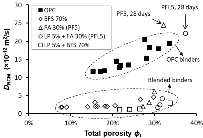
Fig. 5.5 Relationship between chloride migration coefficient D_{\text{RCM}} and total porosity \phi_t for different binders (28~370 days old). All D_{\text{RCM}} - \phi_t plots, except two (PF5 and PFL5 at 28 days), can be divided into two groups: one for OPC binders and the other for blended binders.
