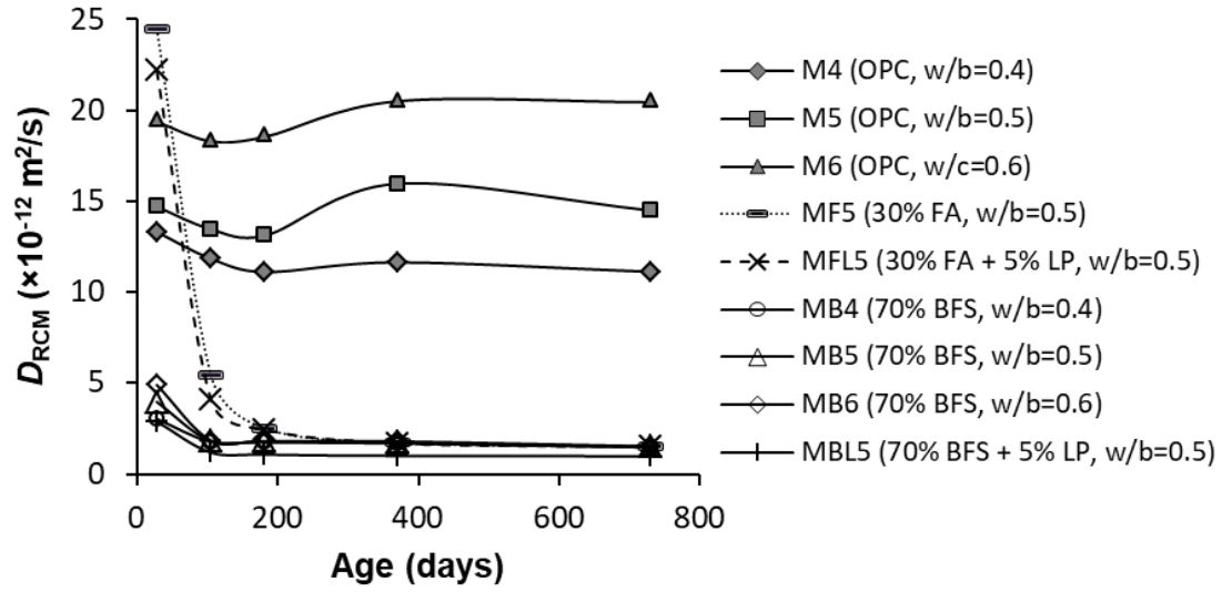
Fig. 5.3 Changes of chloride migration coefficient D_{RCM} with age from 28 days up to 2 years in the OPC and blended mortars.
