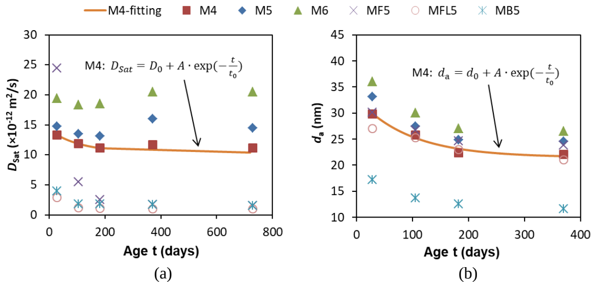
Fig. 8.3 (a) Evolution of the chloride diffusion coefficient D_{\text{Sat}} obtained from RCM tests on saturated specimens. (b) Evolution of the average pore diameter d_a obtained from MIP tests. Mixtures: M4 (OPC, w/b = 0.4 ), M5 (OPC, w/b = 0.5 ), M6 (OPC, w/b = 0.6 ), MF5 (30% FA, w/b = 0.5 ), MB5 (70% BFS, w/b = 0.5 ), MFL5 (30% FA + 5% LP, w/b = 0.5 ).
