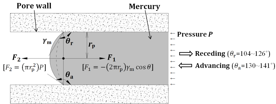
Fig. 3.6 Equilibrium of forces acting inside cylindrical pores.
