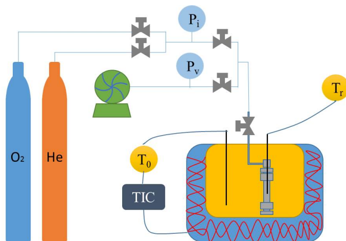
Figure 1: Experimental apparatus
