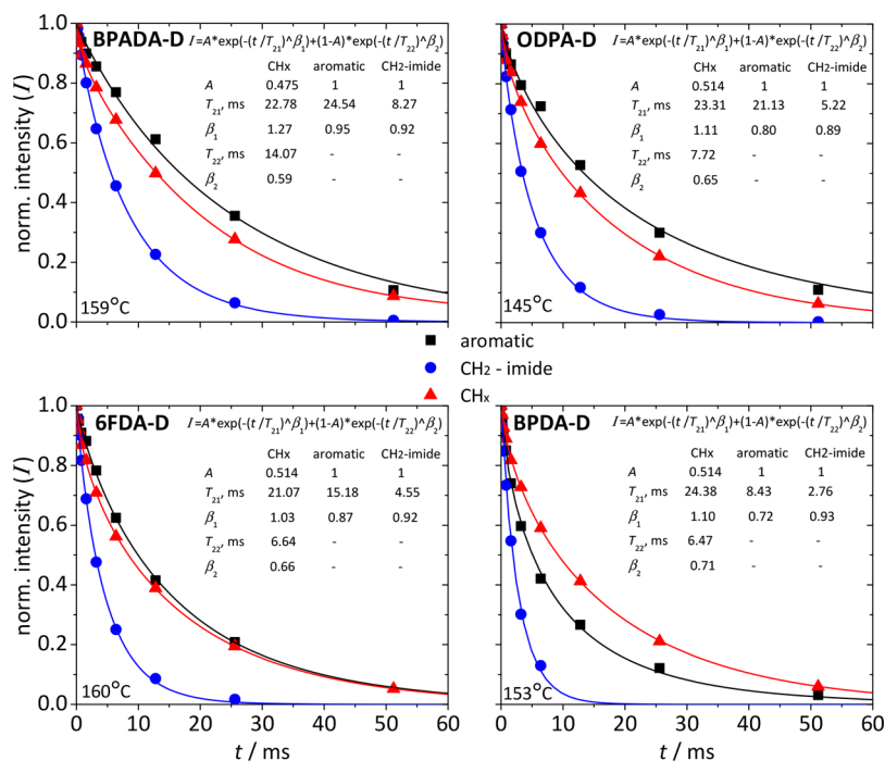
Figure 6. Results of the rotor-synchronized Hahn echo experiments for the four PIs. The corresponding experimental temperatures ( T_{\text{exp}} = T_{\text{tan } \delta \text{ MAX}} + 120 °C) are specified. The solid lines represent the KWW fits (eq 2).
