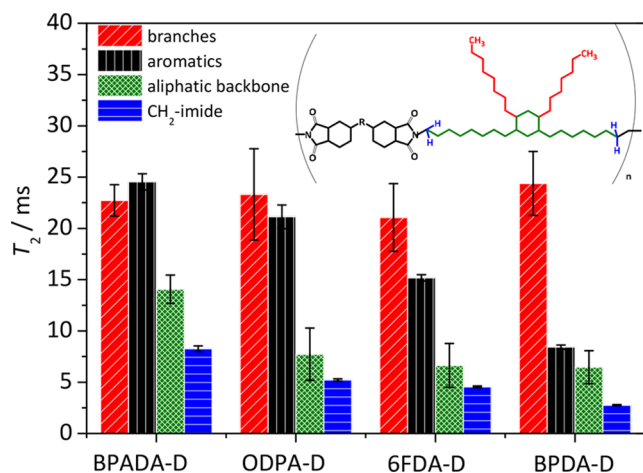
Figure 7. Extracted T_2 relaxation times of the studied PIs measured at T_{\text{exp}} = T_{\text{tan } \delta_{\text{MAX}}} + 120 °C. The absolute T_2 values cannot be compared between different species.
