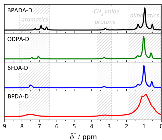
Figure 5. SS NMR one-pulse spectra, magic angle spinning (MAS) at 10 kHz, T_{exp} = T_{\tan \delta \text{ MAX}} + 120 \text{ } ^\circ\text{C} .
