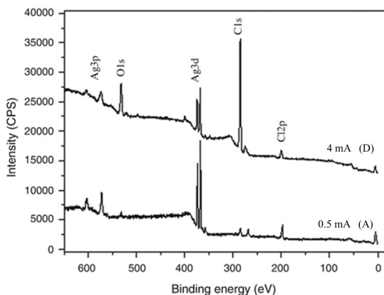
Figure 3.8: Survey XPS spectra for sensors A at 0.5 \text{ mA/cm}^2 and sensor D at 4 \text{ mA/cm}^2 .
