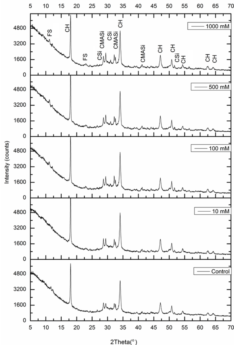
Figure 5.10: XRD pattern of cement paste made of CEM I 52.5N (w/c=0.4) after 300 days of immersion in solutions with different chloride concentration.
