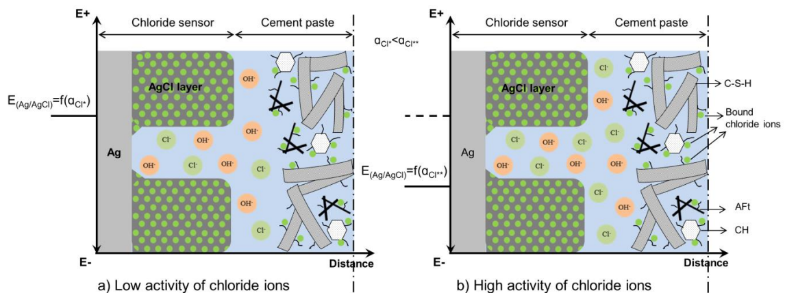
Figure 2.10: Schematic of \text{Ag}/\text{AgCl}/\text{pore solution} interface in chloride-containing cementitious materials, a) low activity of chloride ions, b) high activity of chloride ions. In the presence of chloride ions, the surface of the sensor mainly consists of \text{AgCl} particles. The binding of chloride ions to the hydration products together with the microstructure of cementitious materials affect the activity of the chloride ions at the sensor's surface.
