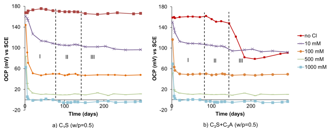
Figure 5.4: The OCP response of chloride sensor in specimens made of cement components, (a) C_3S only and (b) C_3S , C_3A and gypsum, with w/p=0.5 over time.
