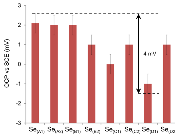
Figure 6.6: OCP response of all sensors after 180-day immersion of specimens in Cl-containing simulated pore solution (SPS).
