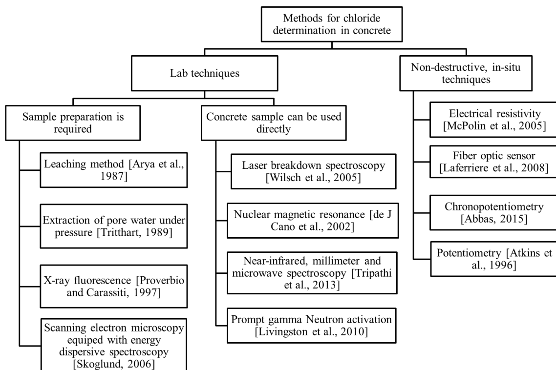
Figure 2.5: An overview of the available techniques for measuring the chloride content in concrete.
