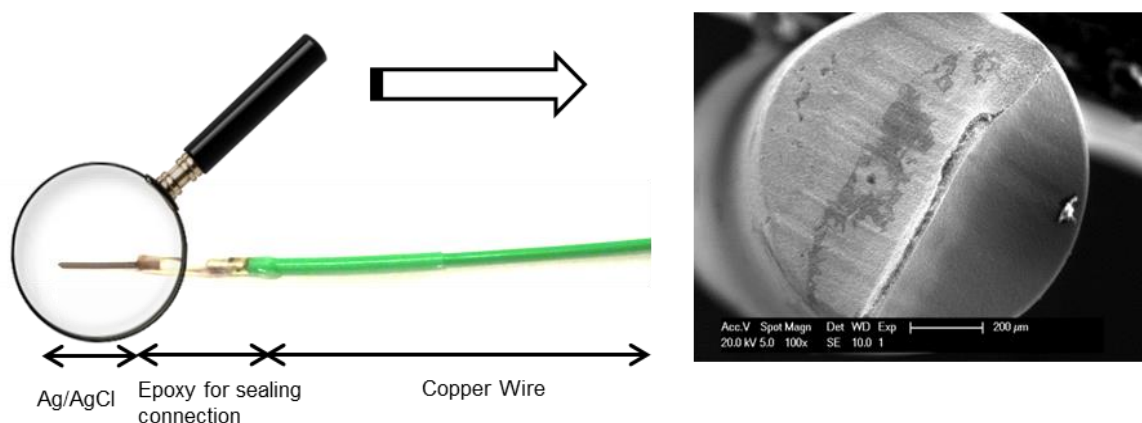
Figure 4.2: The as produced Ag/AgCl chloride sensor.
