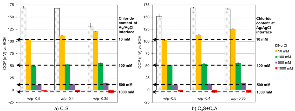
Figure 5.6: The OCP response of chloride sensor after 150-day immersion of (a) C_3S specimens and (b) C_3S+C_3A specimens in solutions with different chloride concentration. The expected response for a A/AgCl interface at different chloride concentration is specified by dashed line.
