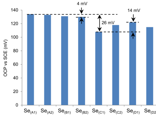
Figure 6.3: OCP response of sensors cast in cement paste cylinders, on the first day of immersion of \text{Se}_{(\text{A1,2})} to \text{Se}_{(\text{D1,2})} in Cl-containing simulated pore solution (SPS).
