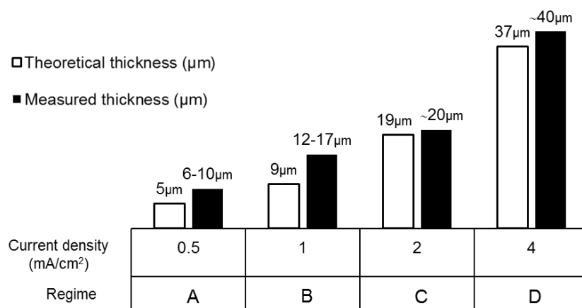
Figure 3.5: One-hour anodization regimes used for sensor preparation and AgCl layer thickness.
