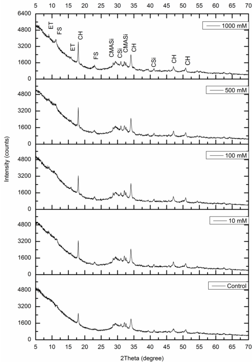
Figure 5.11: XRD pattern of cement paste made of CEM III/A 52.5 N ( w/c=0.4 ) after 300 days of immersion in solutions with different chloride concentration.
