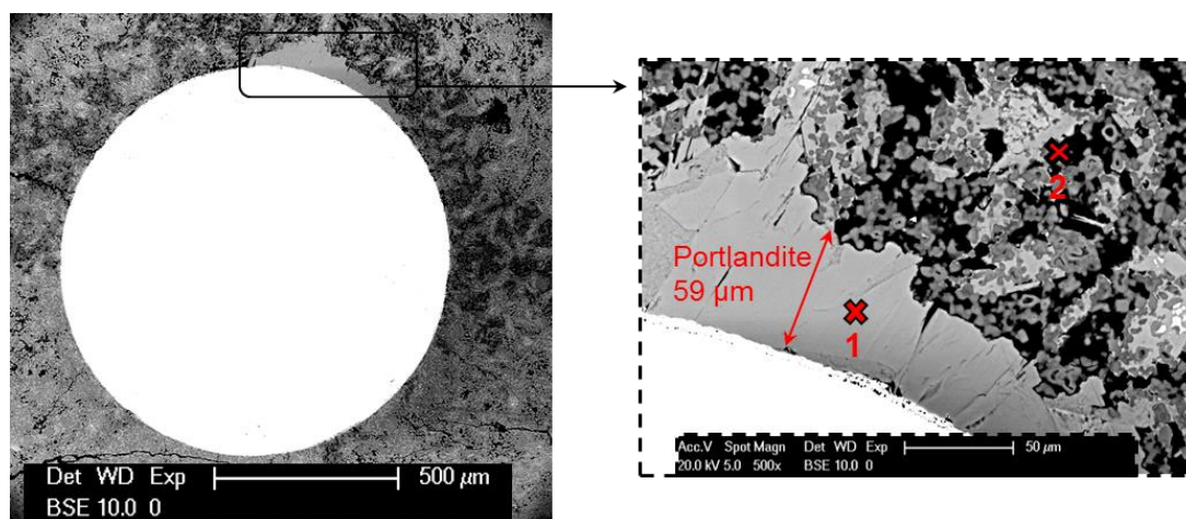
Figure D.1: ESEM images of the cross section of the embedded sensor in C_3S (w/p=0.5) specimen after 300 days of immersion in chloride-free solution. The large crystals of Portlandite can be found occasionally around the sensor. The EDS spectra of the points 1 and 2 are presented in Fig. D.2.
