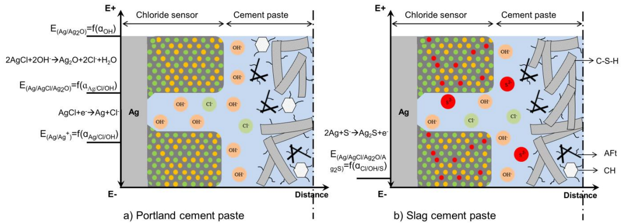
Figure 2.11: Schematic of Ag/AgCl/pore solution interface in chloride-free cementitious materials, a) Portland cement paste, b) slag cement paste. In the absence of chloride ions, a gradual dissolution of the AgCl layer is accompanied by the formation of \text{Ag}_2\text{O} , \text{Ag}^\circ or \text{Ag}_2\text{S} (in case of slag cement concrete) [Graedel, 1992; Femenias et al., 2015]. The formation of these products depends on the concentration of hydroxide and sulfide ions in the medium and the microstructure of cementitious materials at the interfacial zone with the sensor.
