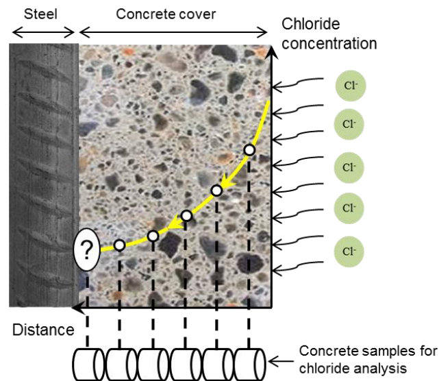
Figure 2.4: Chloride profile in concrete and determination of chloride threshold value.
