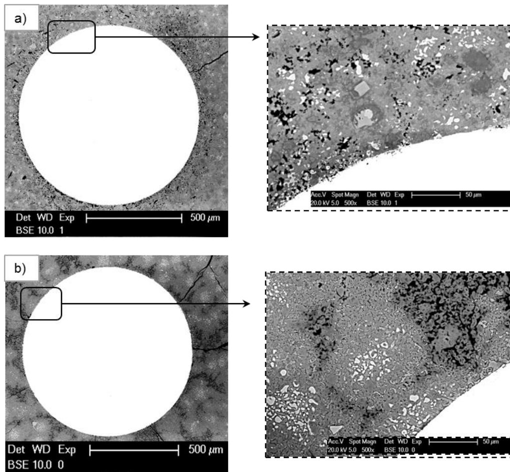
Figure D.6: ESEM images of the cross section of the embedded sensor in a) C_3S+C_3A (w/p=0.35) specimen and b) C_3S (w/p=0.35) specimen after 300 days of immersion in chloride-free solution. The cement matrix in the vicinity of the sensor is denser when compared with the cement matrix in Figs. D.1, D.3 and D.4.
