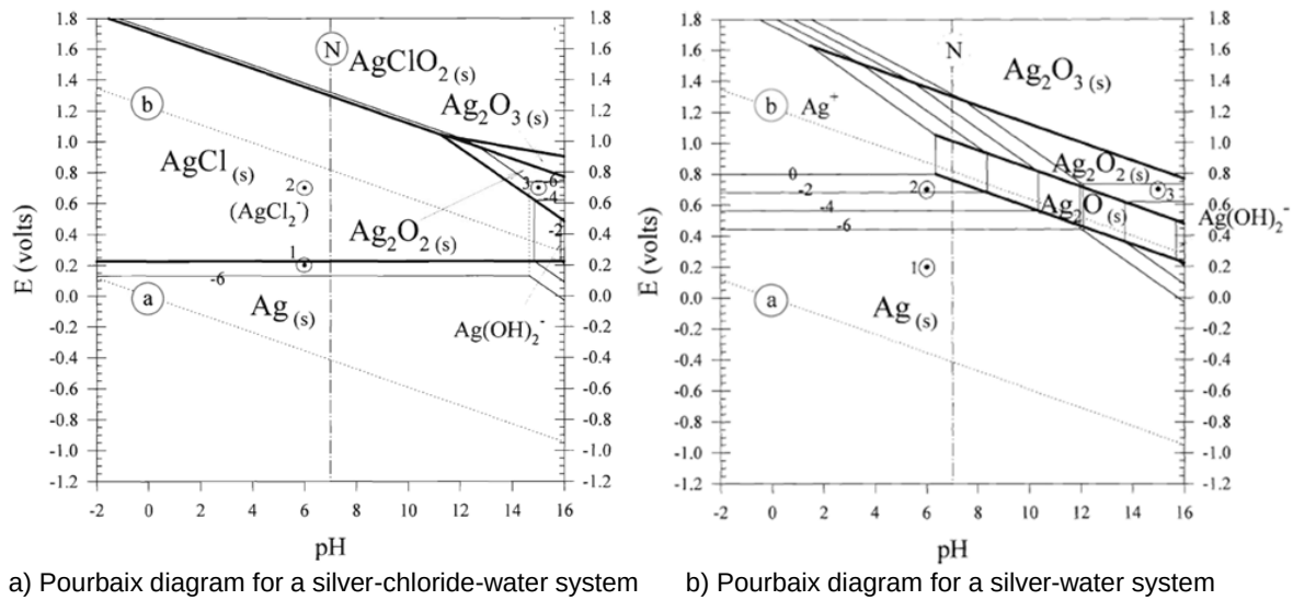
Figure 2.9: a) Pourbaix diagram for a silver-chloride-water system at 25 °C with 1 m chloride concentration and different concentrations of silver ions ( 10^{-6} , 10^{-4} , 10^{-2} m), b) Pourbaix diagram for a Ag-water system at 25°C with different concentration of silver ions from 1 to 10^{-6} m. The potentials are vs. SHE reference electrode [Winston, 2000].
