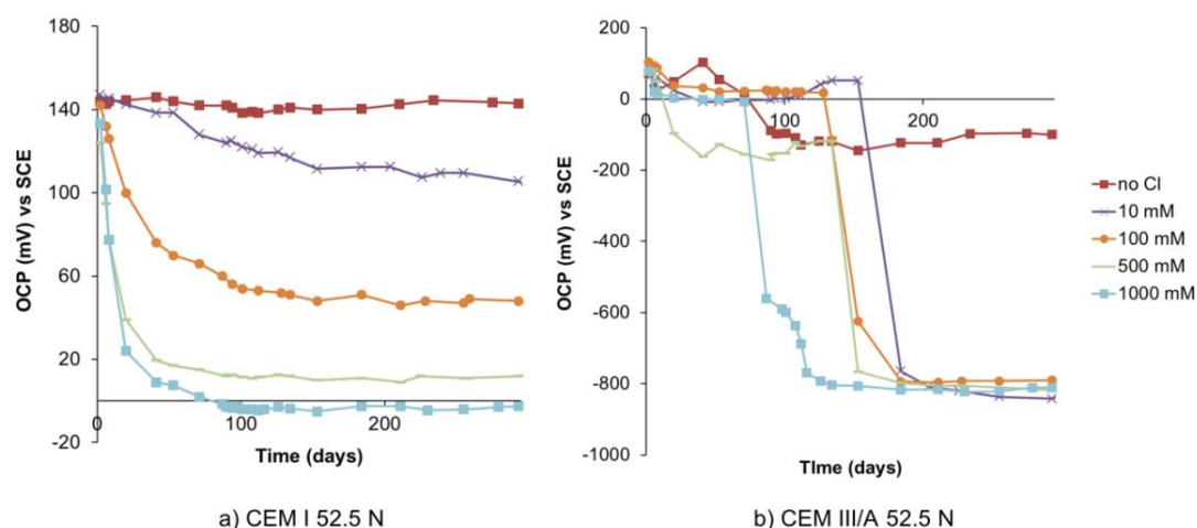
Figure 5.7: The OCP response of chloride sensor in cement paste made of (a) CEM I 52.5 N and (b) CEM III/A 52.5 N with w/c=0.4 over time.
