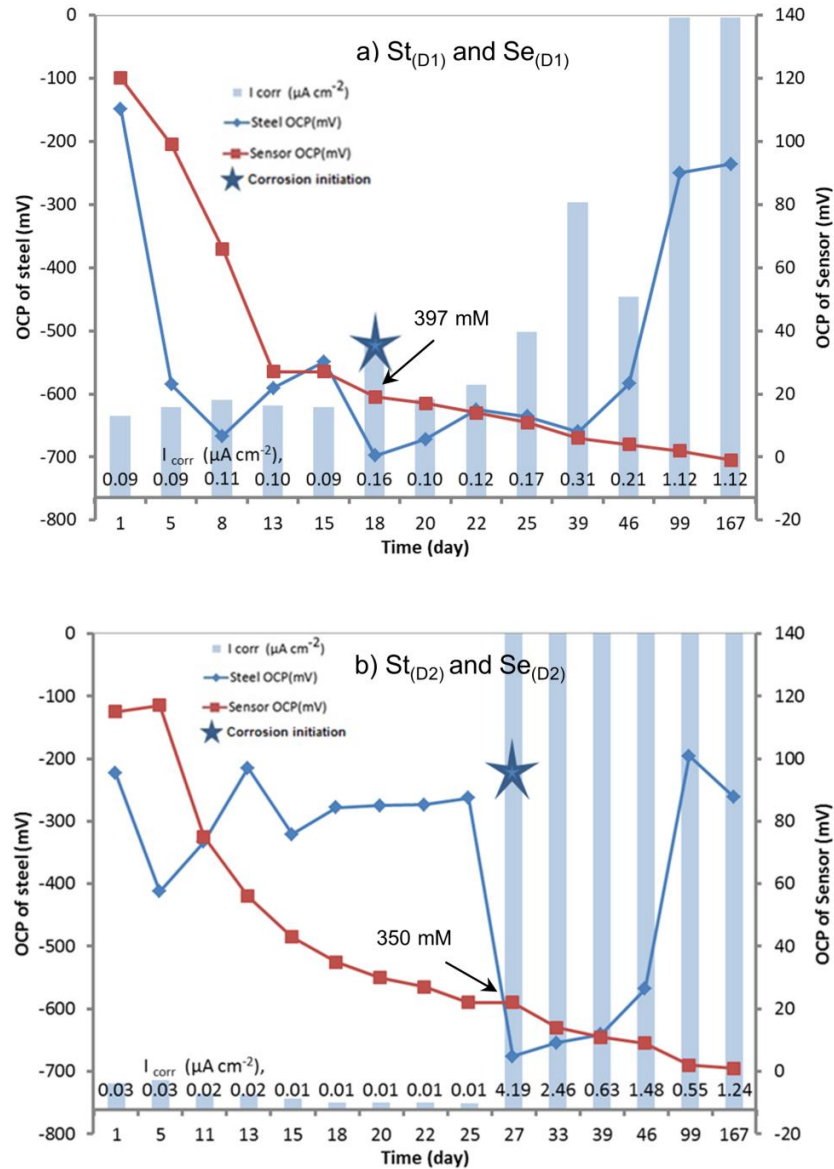
Figure 6.11: Corrosion current density ( I_{corr} ) of steel rods in addition to the OCP of steel and sensor at a certain time over immersion period: a) St_{(D1)} and Se_{(D1)} ; b) St_{(D2)} and Se_{(D2)} .
