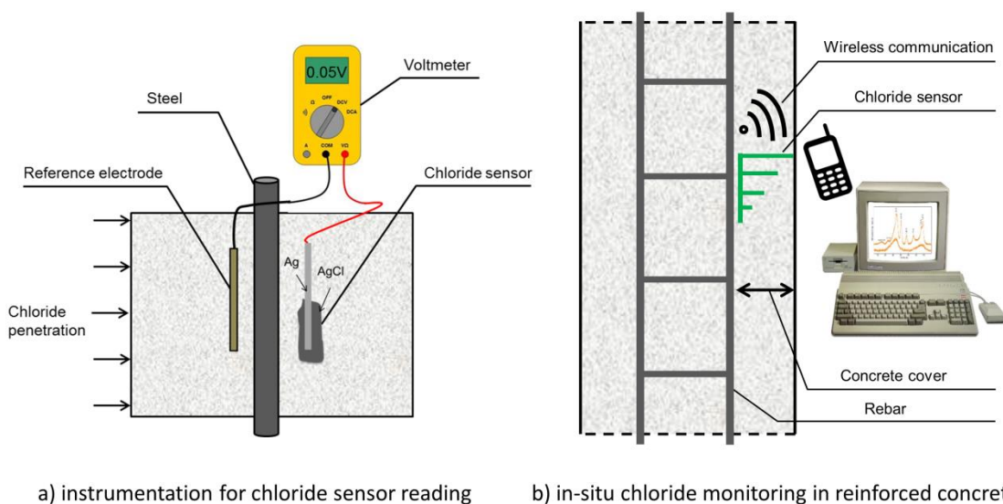
Figure 1.1: Schematic illustration of the instrumentation for chloride sensor readings in reinforced cement-based material.
