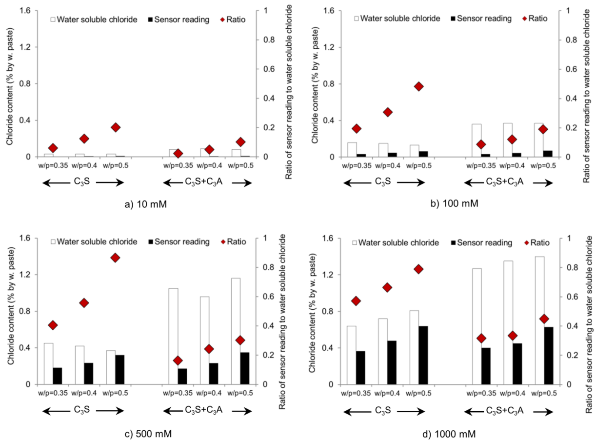
Figure 5.15: The water-soluble chloride, sensor reading of the free chloride content and the ratio of sensor reading to water-soluble chloride for C_3S and C_3S+C_3A specimens after 300 days of immersion in solutions with different chloride concentration.
