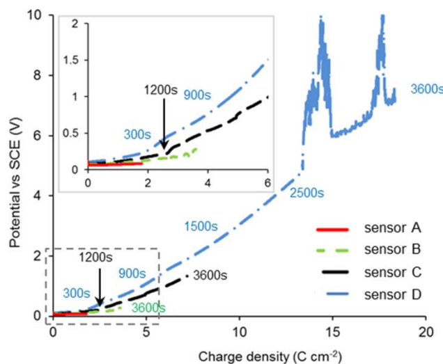
Figure 3.11: Overpotential vs. charge density during anodic formation of AgCl on a Ag wire in 0.1 M HCl in different current density regimes of 0.5 mA/cm 2 (sensor A), 1 mA/cm 2 (sensor B), 2 mA/cm 2 (sensor C) and 4 mA/cm 2 (sensor D).
