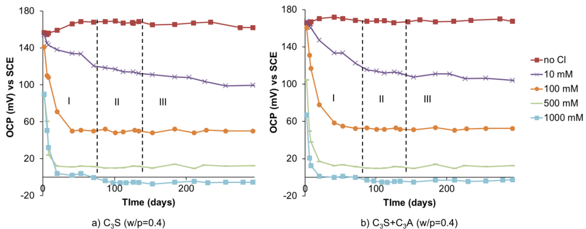
Figure 5.3: The OCP response of chloride sensor in specimens made of cement components, (a) C_3S only and (b) C_3S , C_3A and gypsum, with w/p=0.4 over time.
