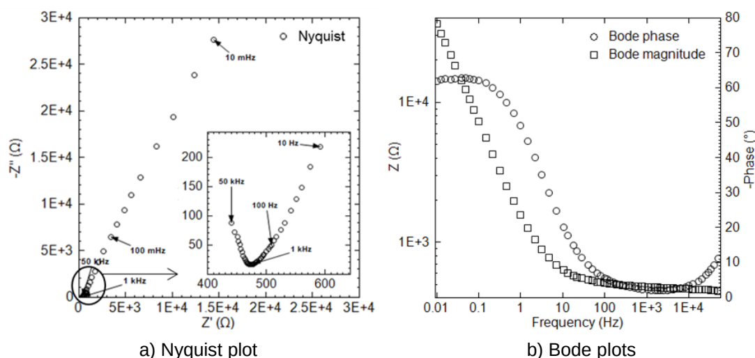
Figure 6.7: EIS response of steel rod cast in cement paste cylinder and immersed in Cl-containing simulated pore solution (SPS).
