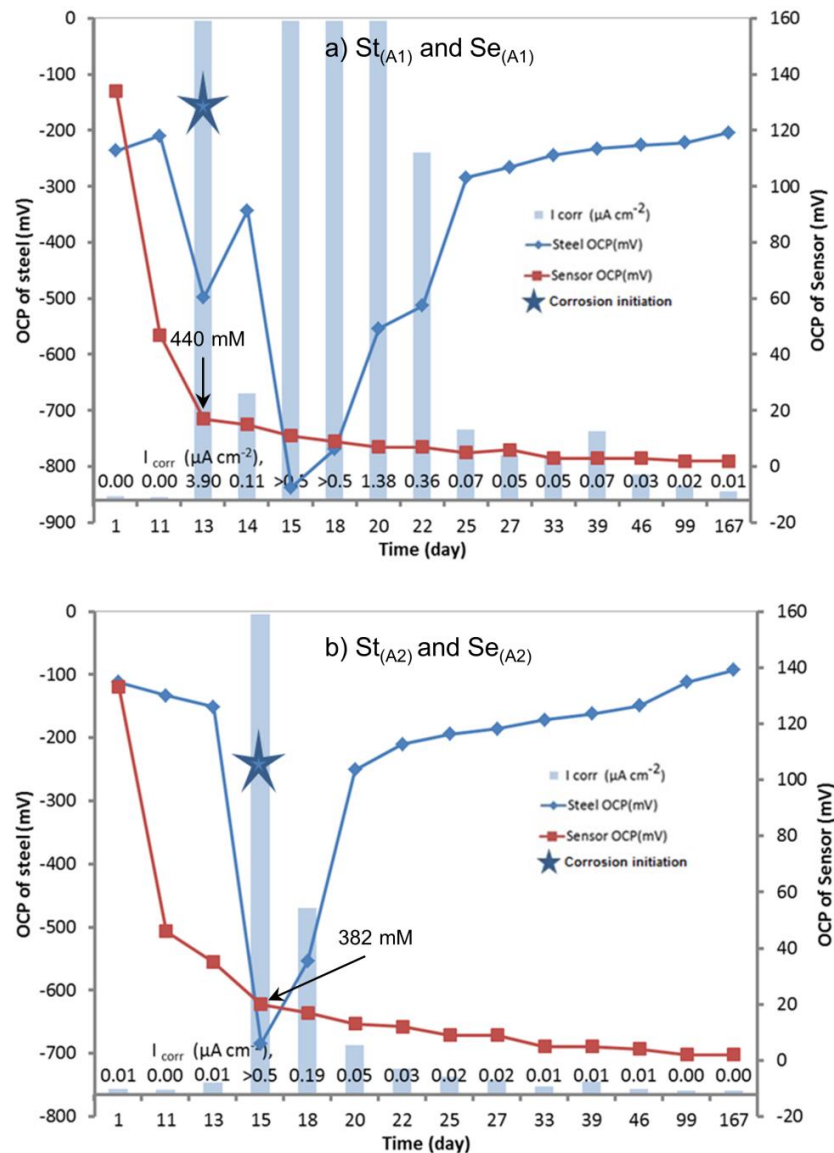
Figure 6.9: Corrosion current density ( I_{corr} ) of steel rods in addition to the OCP of steel and sensor at a certain time over immersion period: a) St_{(A1)} and Se_{(A1)} ; b) St_{(A2)} and Se_{(A2)}
