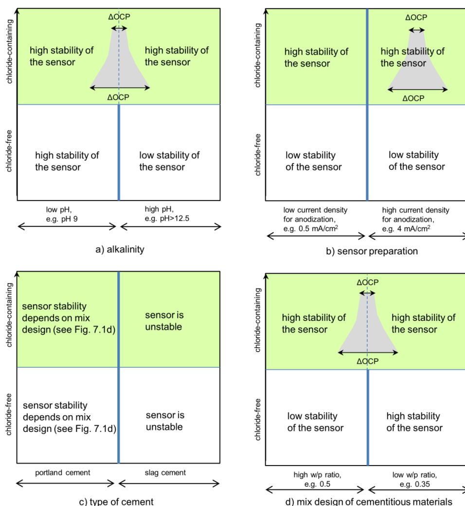
Figure 7.1: Schematic representation of the influence of studied parameters on the performance of the chloride sensor: a) alkalinity of the solution; b) sensor preparation; c) type of cement; d) mix design.
