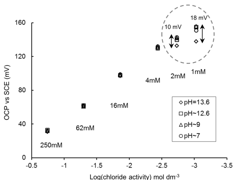
Figure 4.7: The effect of pH on the OCP response of the chloride sensor.
