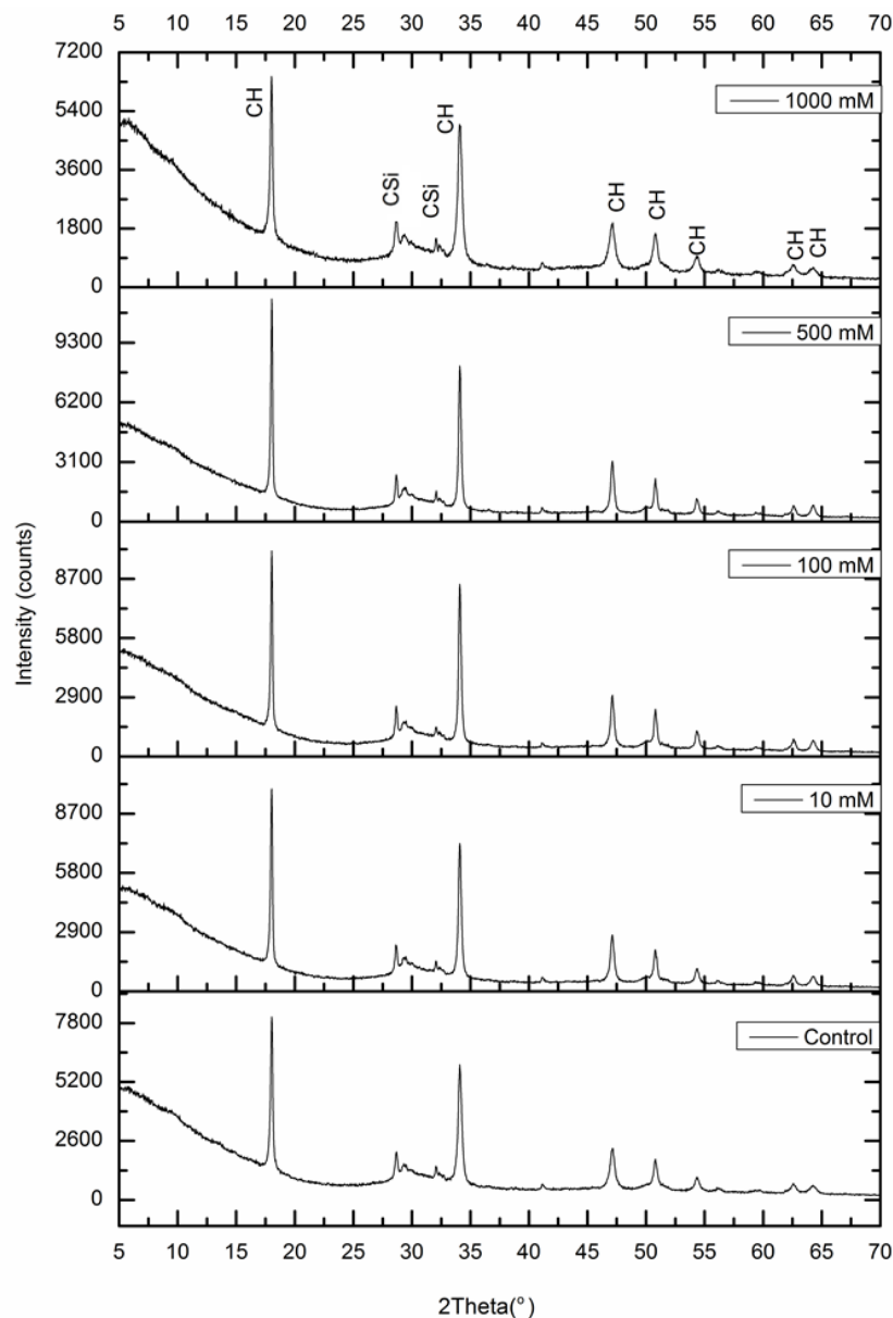
Figure 5.8: XRD pattern of C_3S (w/p=0.4) paste after 300 days of immersion in solutions with different chloride concentration.
