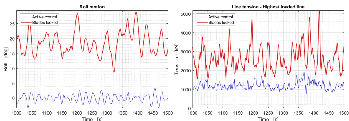
Figure 7. Time traces of roll and mooring line tension for the two control settings during survival
