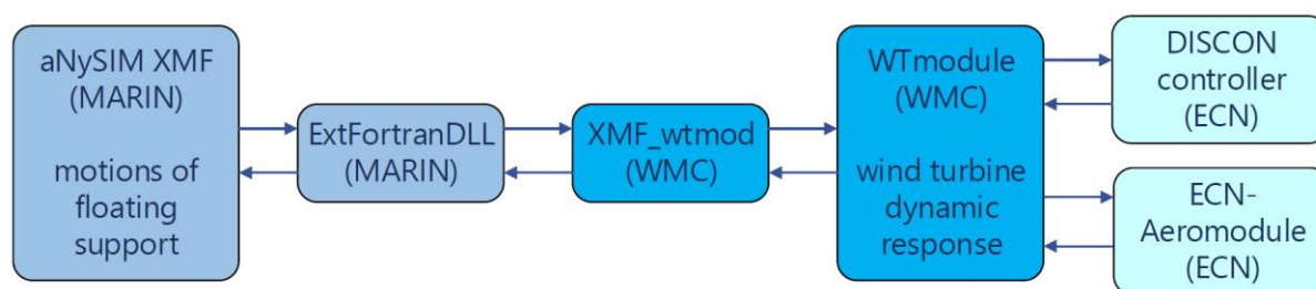
Figure 6. Coupled software for floating VAWT analysis
