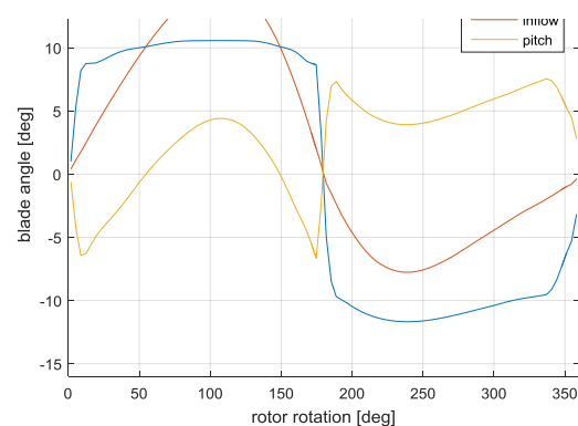
Figure 3. Blade pitch trajectory
