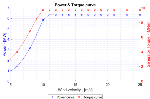
Figure 4. Generator power and torque curves
