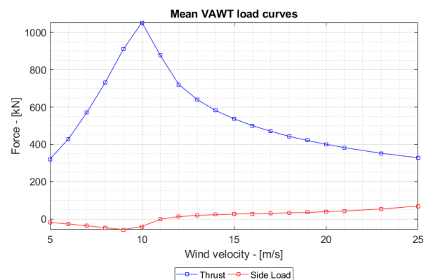
Figure 5. Thrust and side load curves
