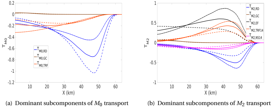
Figure 4.23: Dominant subcomponents of the M_0 (left panel) and M_2 (right panel) transport components for shallowing by 1 m ( \delta H_{\max} = -1 m, dashed line) and deepening ( \delta H_{\max} = 1 m, dotted line). The solid lines denote the nominal case i.e., \delta H_{\max} = 0 m.
