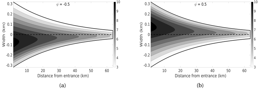
Figure 4.7: Laterally asymmetric bed profiles for \psi = -0.5 (left panel) and \psi = 0.5 (right panel). For \psi = -0.5 , the bed profile is skewed to the left when viewed from the river side to the seaward side and for \psi = 0.5 , skewed to the right. The units in the colorbar are m.
