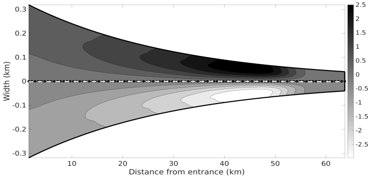
Figure 4.6: Lateral diffusive transport T_{\text{diff}}^{ya} . The black stars in the middle indicates the middle of the channel ( y = 0 ) and the black solid lines at the sides, the domain boundaries. The white dashed line in the middle indicates the zero contour of the lateral diffusive transport. The white dashed line for the zero contour overlaps with the black stars in the middle indicating a clear partition between the negative transport in the lower part (below y = 0 ) and positive transport in the upper part (above y = 0 ) of the channel.
