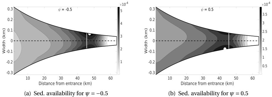
Figure 4.8: Sediment availability for positively skewed bed profile with \psi = -0.5 (left panel, a) and negatively skewed bed profile with \psi = 0.5 (right panel, b). The white circle denotes the location of maximum sediment availability. The white line denotes the x -location of the maximum sediment availability for the reference case with \psi = 0 .
