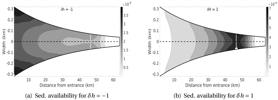
Figure 4.18: Availability of fine sediments at the bottom for fall (left panel) and rise (right panel) of the sea level. The white circle denotes the location of maximum sediment availability for the current case and white line, the x-location of maximum availability for the reference case. The sediment availability is a dimensionless quantity and hence no units are associated with the colorbar.
