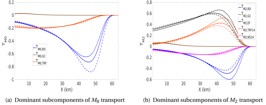
Figure 4.22: Dominant width-averaged subcomponents of the M_0 (left panel) and M_2 (right panel) transport components for bed profiles with \psi = -0.5 (dashed line), \psi = 0 (solid line) and \psi = 0.5 (dotted line).
