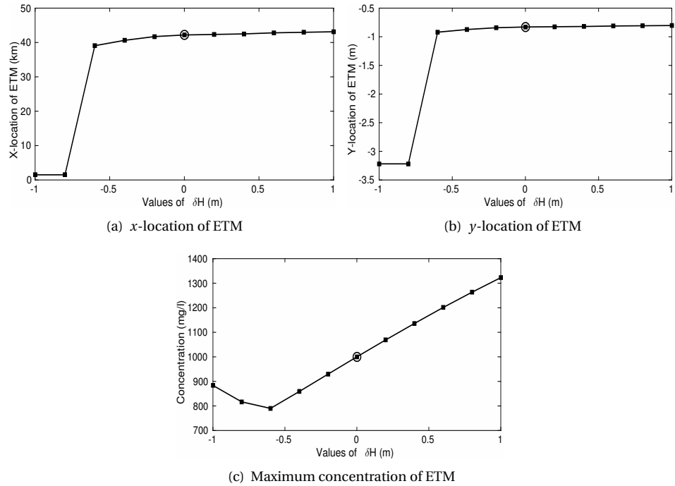
Figure 4.15: Influence of shallowing and deepening on the location and strength of ETM. The top left panel shows the x -location or the distance from the entrance of the ETM and the top right panel the y -location of the ETM. The bottom panel shows the strength of the ETM in terms of maximum suspended sediment concentration at the surface. In all the panels, solid black squares indicate the model results and black circle indicates the data for the reference case.
