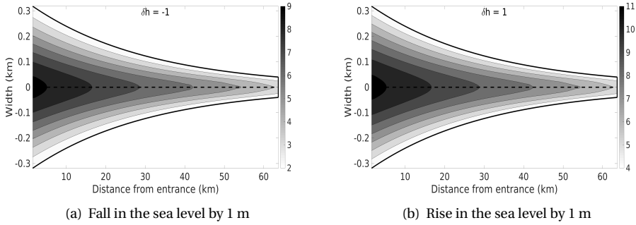
Figure 4.17: Bathymetric profiles due to fall (left panel) and rise (right panel) in the sea level. For fall in the sea level, \delta h = -1 is used and for rise in the sea level \delta h = 1 . The units in the colorbar are m.
