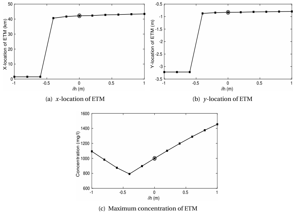
Figure 4.20: Influence of changes in the sea level ( \delta h ) on the location and strength of ETM. The top left panel shows the x-location or the distance of the ETM from the seaward side and the top right panel , the y-location of the ETM. The bottom panel shows the strength of the ETM in terms of maximum suspended sediment concentration at the surface. In all the panels, solid black squares indicate the model results and black circle indicates the reference case.
