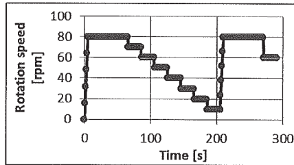
Figure 2. Rotational velocity profile applied in rotational rheometry
