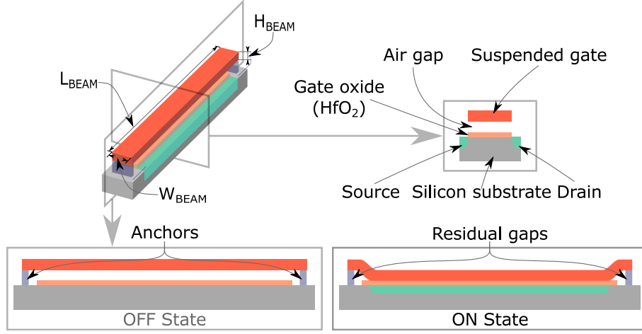
Figure 3.1: NEMFET's geometry [8].
