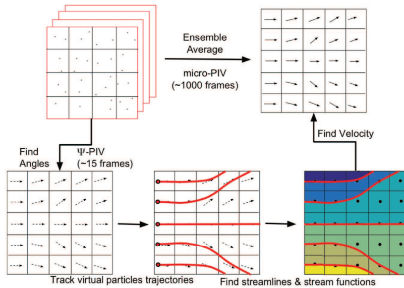
Fig. 2 Principal difference between PIV & \Psi -PIV algorithm
