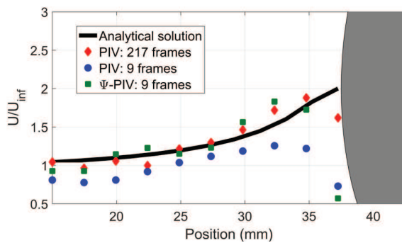
Fig. 6 Measured velocity distribution by PIV, \Psi -PIV around a cylinder (grey shaded region shows the left edge of the cylinder) and compared with the theoretical distribution which is calculated assuming ideal flow conditions
