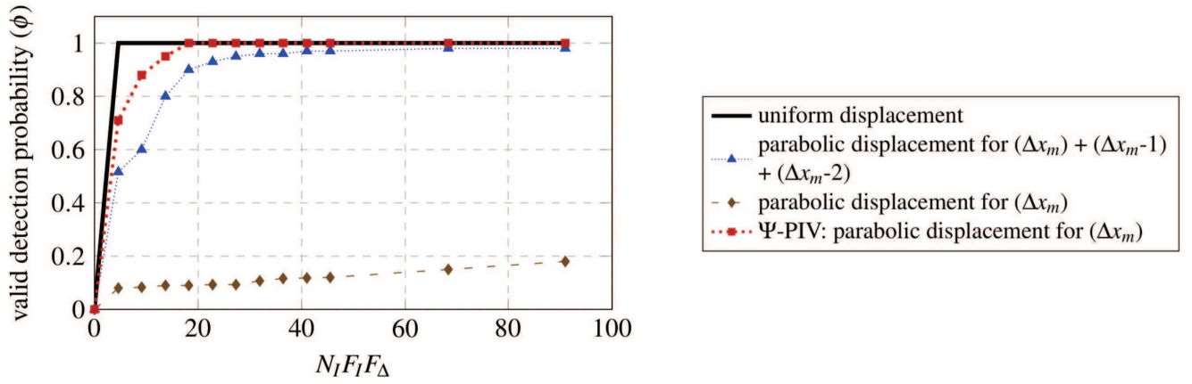
Fig. 3 The detection probability for the displacement correlation peak as a function of mean number of particle within an interrogation window and compared with the results of uniform displacement.
