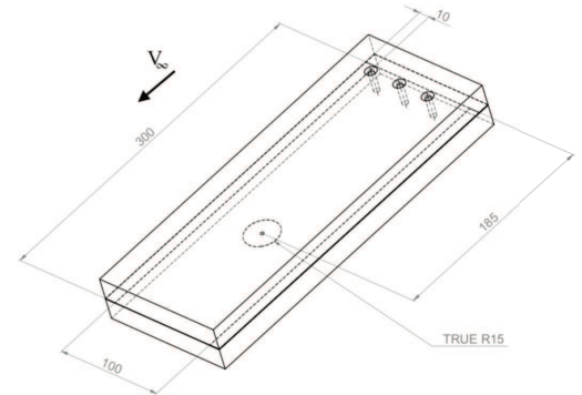
Fig. 4 Schematic of the test setup showing the flow direction & the three inlet holes
