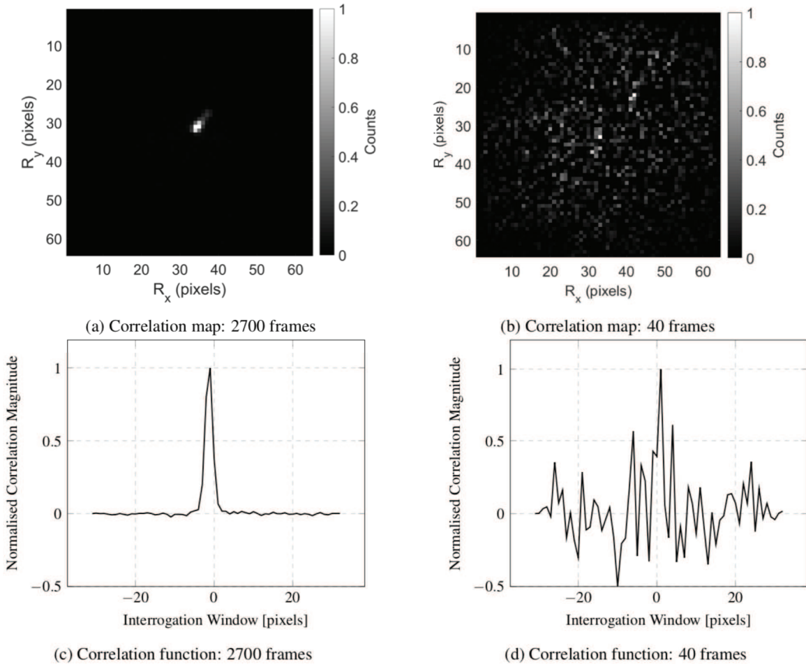
Fig. 1 Ensemble cross-correlation for 32 \times 32 px interrogation window where the flow direction was calculated as 63^\circ for 2700 averaged images & 40 averaged images.
