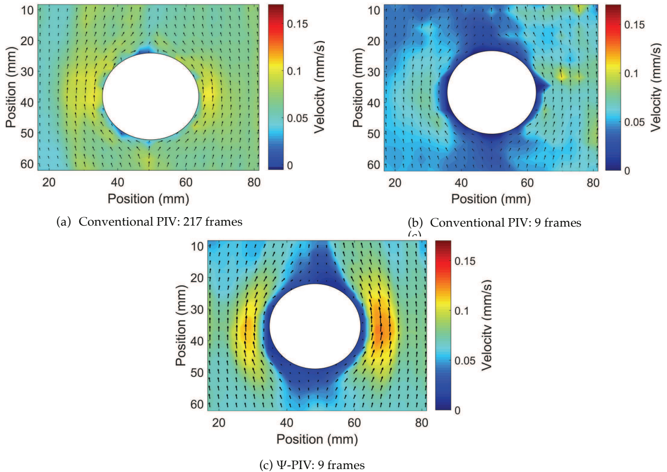
Fig. 5 Results of flow around a cylinder in a Hele-Shaw cell
