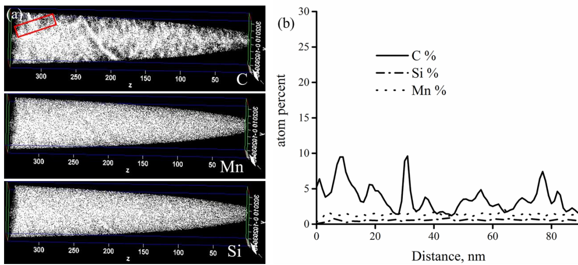
Fig. 4.12: The 3D element maps of APT needle taken in WEL, ~2 μm beneath the rail surface (a) and the composition quantifications of volumes in the empty rectangle in (b).
