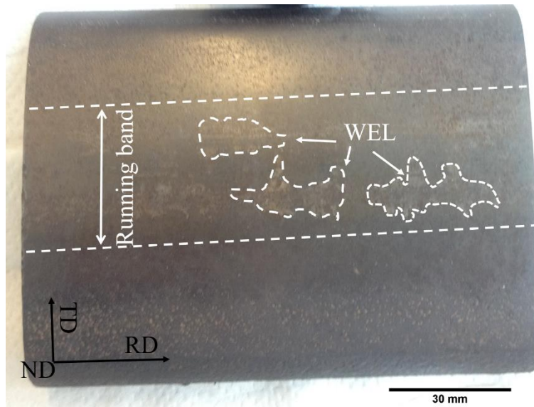
Fig. 3.4: Overview of rail surface after careful grinding and slight etching with 2% Nital. The WEL can be identified by color and part of WEL is indicated by arrows in the photo.
