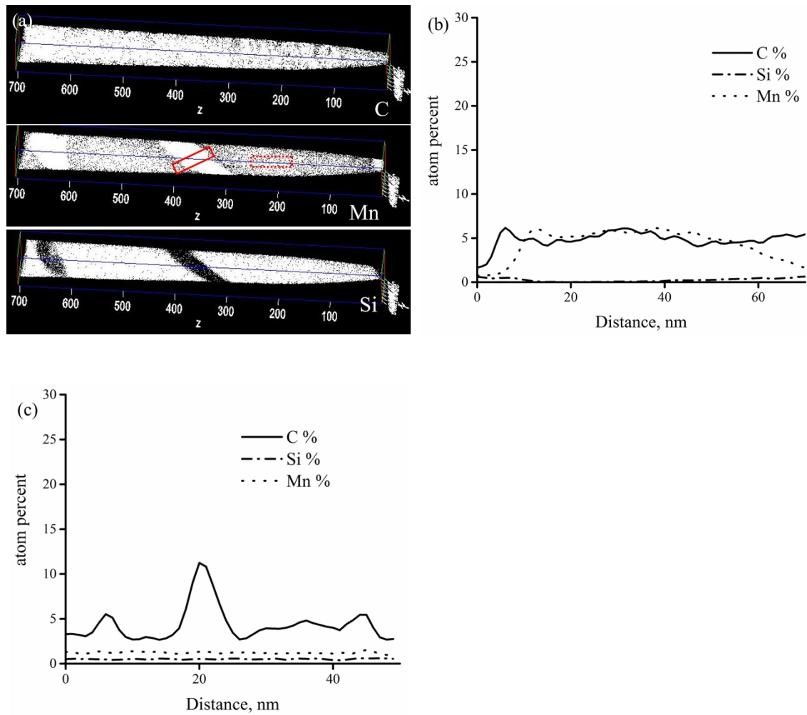
Fig. 4.13: The 3D element maps of APT needle taken in WEL, ~10 μm beneath rail surface (a) and the composition quantifications of volumes in the solid rectangle, in (b), and the dotted rectangle in (c) respectively.
