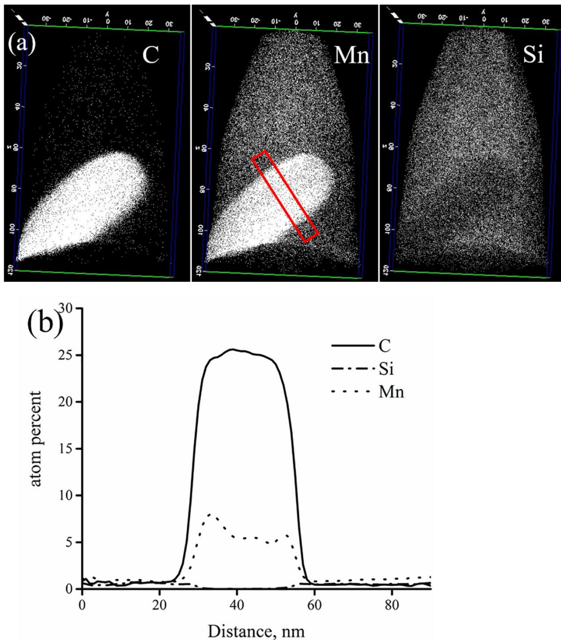
Fig. 4.11: The 3D element maps in the APT needle taken from pearlite \sim 3 \mu\text{m} beneath WEL (a) and the composition quantifications of volumes in the empty rectangle is shown in (b).
