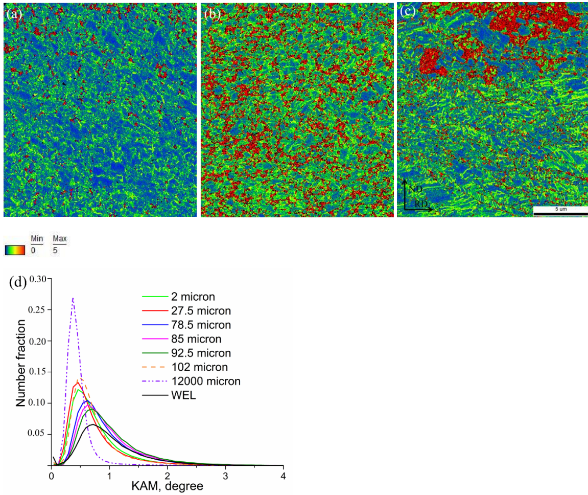
Fig. 7.7 The KAM maps of (a) surface BEL area, (b) BEL zone 80 \mu\text{m} beneath the rail surface and slightly above the BEL/pearlite boundary. (d) The KAM plot of areas in the BEL, deformed pearlite and the undeformed pearlite region. KAM plot of WEL in [6] is added for comparison.
