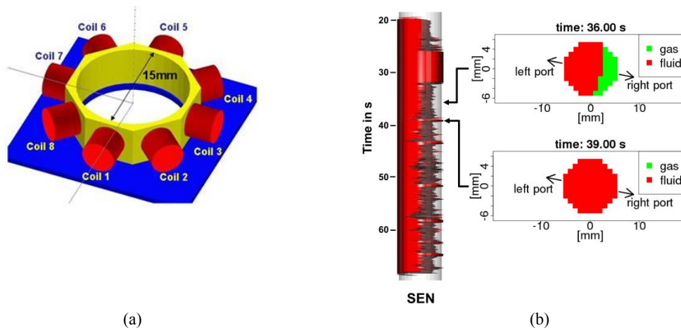
Fig 3.: Schematic (a) of an MIT sensor and reconstructed argon/GaInSn distribution (b) in the SEN at the Mini-LIMMCAST facility (see [8])
