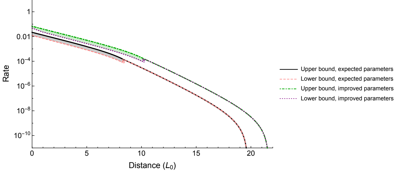
FIG. 4. Upper- and lower bounds on the secret-key rate with a quantum repeater as a function of the distance in units of L_0 = 0.542 km. The repeater is positioned half-way between Alice and Bob. The curves correspond to the expected and improved parameters with optimised cut-off. The improved parameters correspond to setting p_{ps} = p_{em} = 0.6 and F_{gm} = 0.97 . For high losses, the upper- and lower bounds become essentially tight. For this reason, the upper bound on the achieved rate forms a reliable estimate of the secret-key rate.
