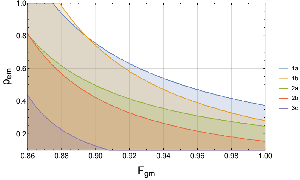
FIG. 11. Contour plot of regions of F_{\text{gm}} versus p_{\text{em}} with the expected parameters where the benchmarks listed in Table I can be surpassed. The contour lines correspond to the parameters that achieve the corresponding benchmarks while the parameter regimes above the curves allow us to surpass them. The data is plotted for the distance of 9.6L_0 , where L_0 = 0.542 km.
