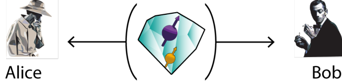
FIG. 3. Single sequential quantum repeater based on an electron spin associated with an NV (purple) and ^{13}\text{C} nuclear spin (orange) in diamond. The previous quantum memories \text{QM}_{1,2} are now represented by the electron and nuclear spin respectively. The optical interface of the NV is strongly Purcell-enhanced by an optical cavity with low-mode volume and allows for efficient photon transmission to Alice and Bob.
