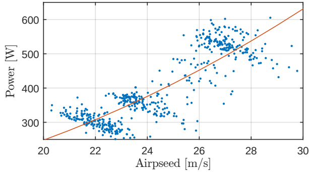
Figure 7: Power versus airspeed during outdoor test flight.
