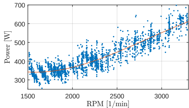
Figure 6: Power required to fly a 22\text{ m/s} at various RPM.
