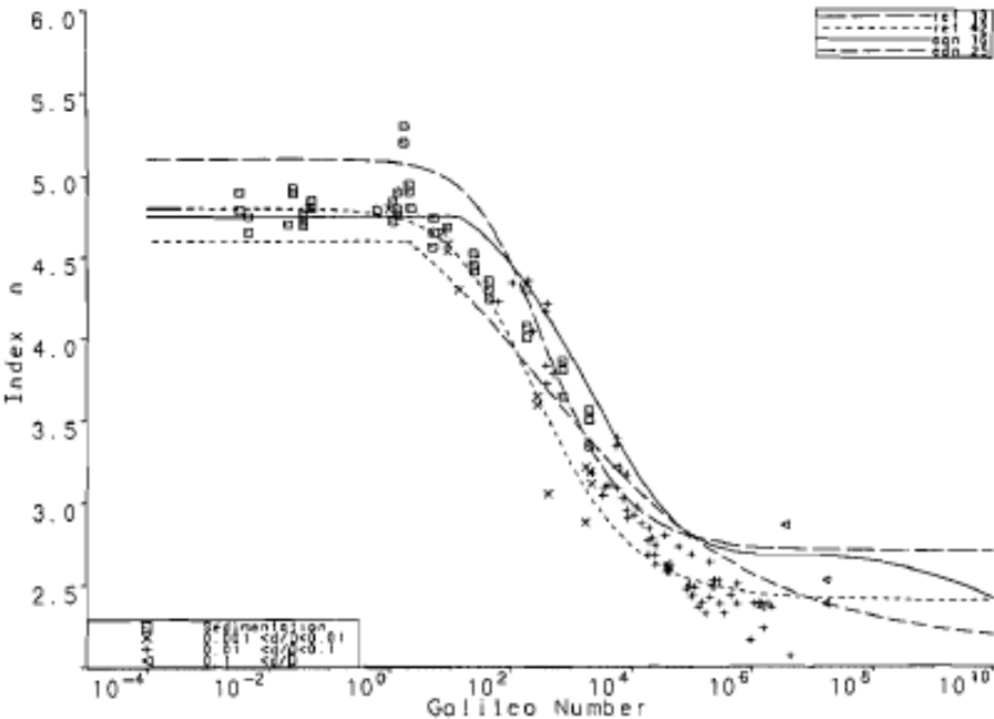
FIGURE 5 Comparison of published correlations with experimental values of index n .
