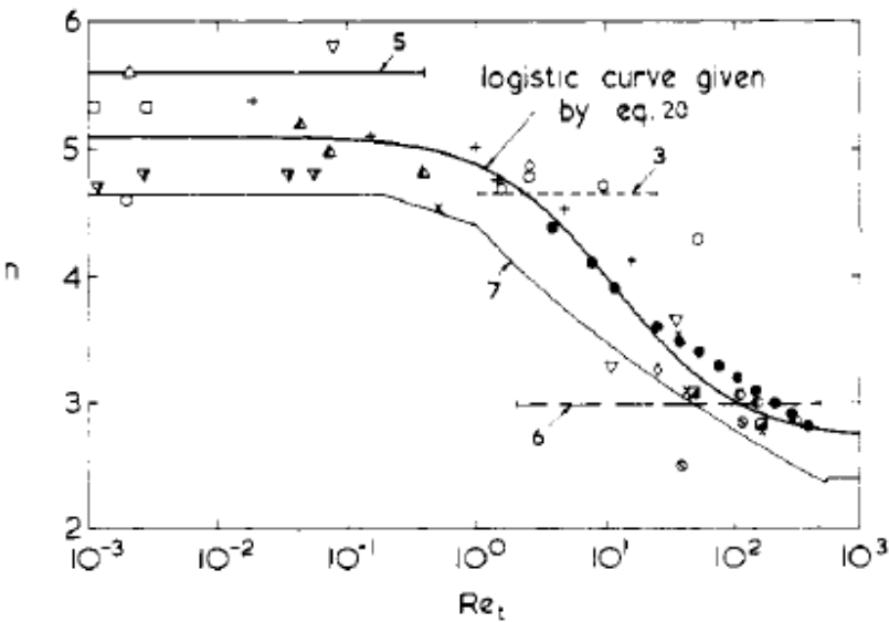
Figure 8. Variation of exponent n with Reynolds number. (See Table I for explanation of symbols; See Table III for key to different curves.)
