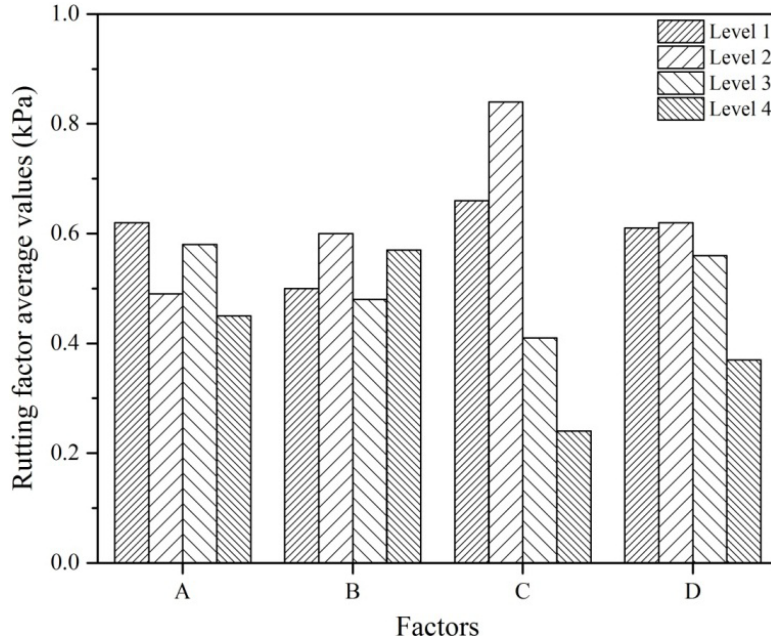
Fig. 11. Rutting factor average values at different levels for different factors.
