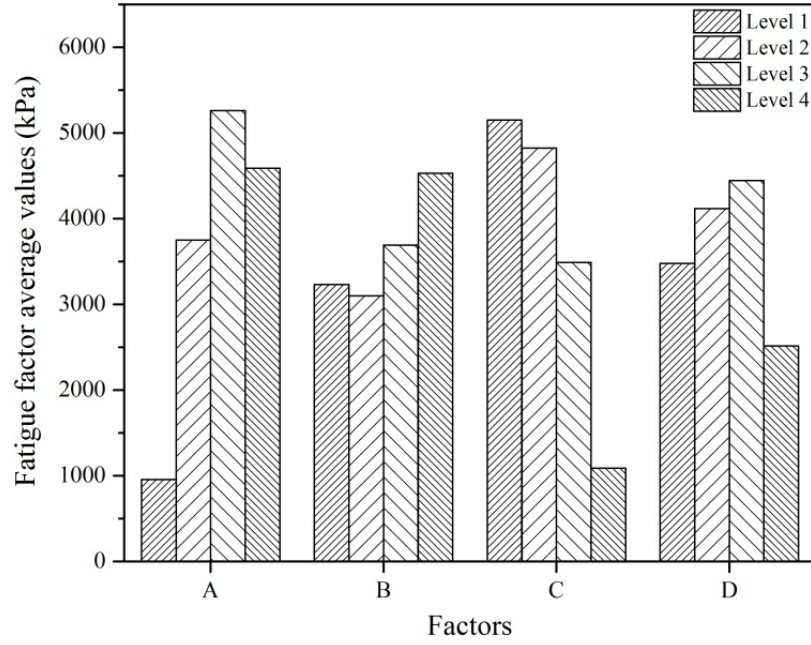
Fig. 12. Fatigue factor average values at different levels for different factors.
