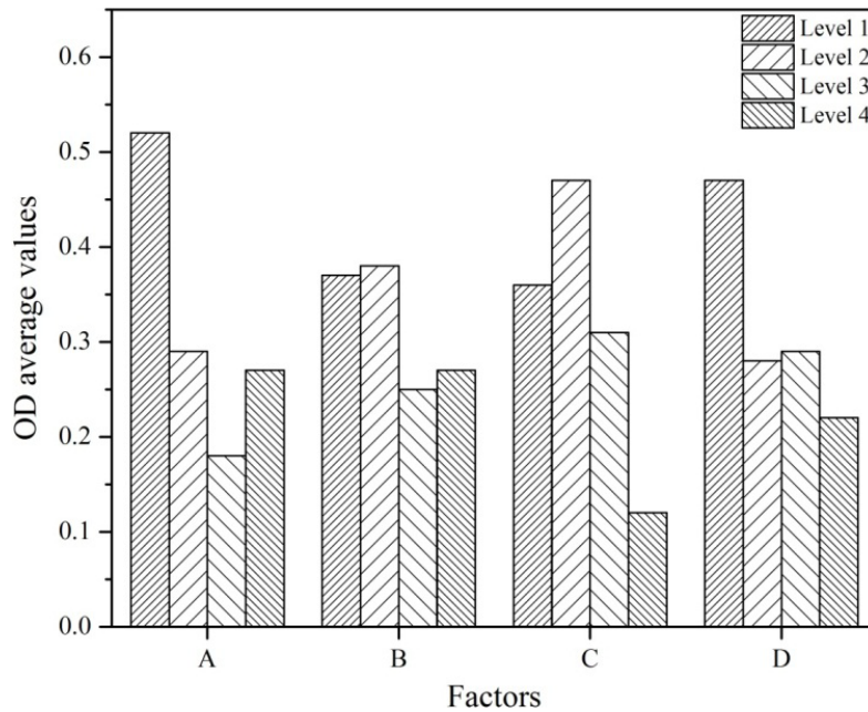
Fig. 13. Overall desirability average values at different levels for different factors.
