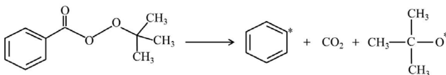
(b) Decomposition of TBPB
