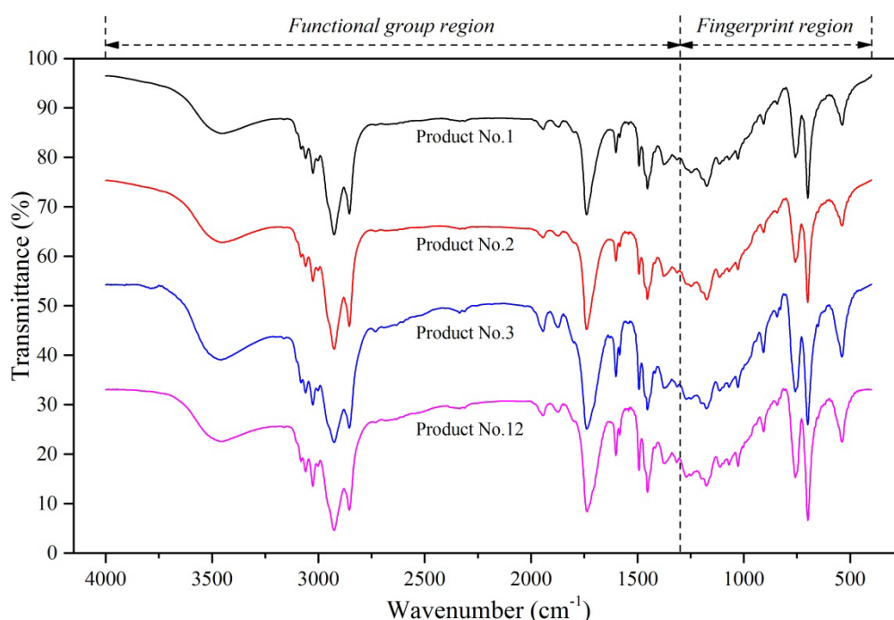
Fig. 7. IR spectra of typical bio-bitumen products.
