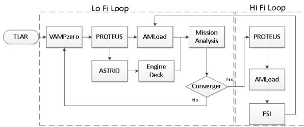
Fig. 2 : MDA Workflow.
