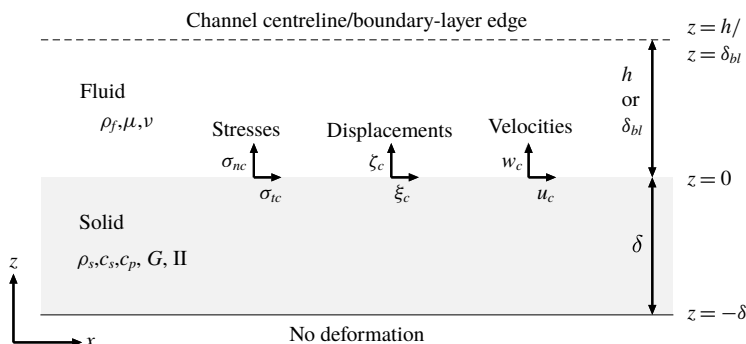
FIGURE 1. Sketch of the analytical problem. The grey layer represents a solid of thickness \delta . A turbulent channel or boundary-layer flow exerts fluctuating tangential stresses \sigma_{tc} and normal stresses \sigma_{nc} on the coating surface. The stresses induce the surface displacements \xi_c and \zeta_c , as well as the surface velocities u_c and w_c .
