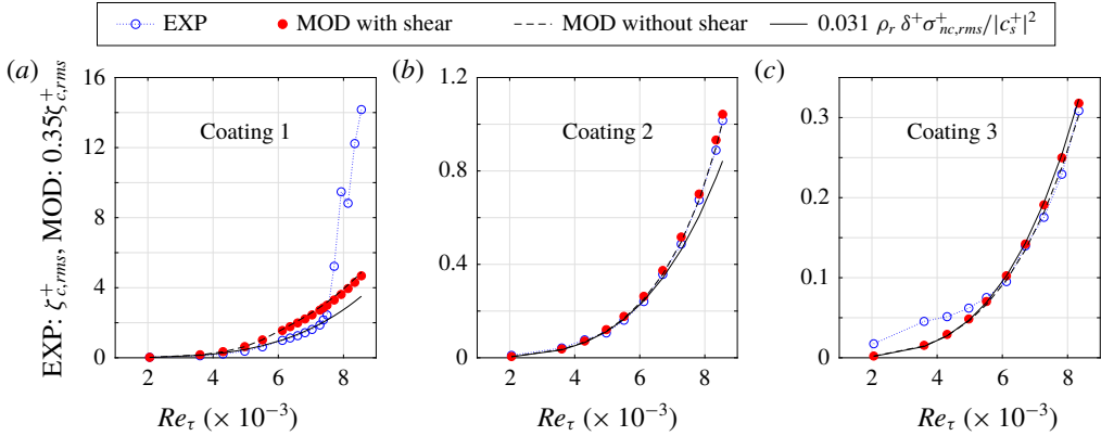
FIGURE 14. (Colour online) The measured and modelled vertical surface displacement as functions of the Reynolds number for three different coatings mentioned in table 2. As explained in the text, the figures display \zeta_{c,rms}^+ for the experiments and 0.35\zeta_{c,rms}^+ for the model. Two model results are shown, one with shear ( E_{\sigma_{nc}} = 0.28E_{\sigma_{nc}} ) and another without shear ( E_{\sigma_{nc}} = 0 ). The continuous line represents a simple analytical relation, with \sigma_{nc,rms}^+ estimated from (5.4).
