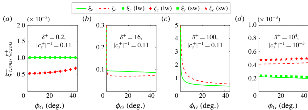
FIGURE 10. (Colour online) Horizontal and vertical surface displacement as functions of the loss angle \phi_G for four parameter sets (see title, corresponding to the four dots in figure 6). The other parameters are Re_\tau = 720 , \rho_r = 1 , \nu_{pr} = 0.45 . The long-wave (lw) and short-wave (sw) results are included in panels (a) and (d), respectively.
