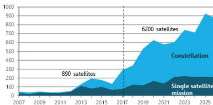
Figure 5-1 | Small satellite (< 500 kg) launches and projected launches [8]
