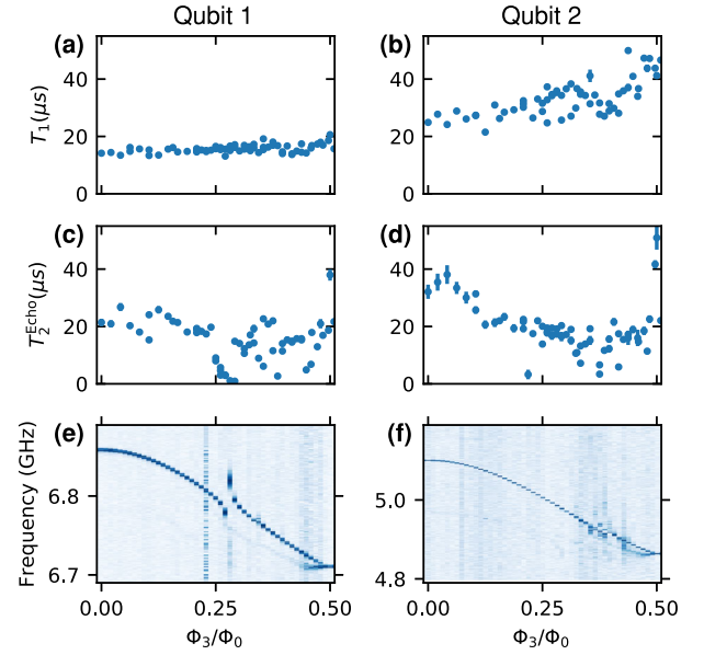
Fig. 4 Observation of high qubit coherence vs coupler flux bias. a, b T_1 measurements showing high energy-relaxation times (15–40 μs) for the whole range of coupler bias, with the qubits detuned at their top and bottom sweetspots. c, d Respective measurements of T_2^{\text{Echo}} decay times vs \Phi_3/\Phi_0 . High coherence is observed except for the points where a lower sloshing circuit mode crosses the qubits (see text for details). e, f Respective spectroscopy of both qubits vs \Phi_3/\Phi_0 . As the inductance of the coupler is varied the qubit frequencies change as expected from theory. The 0–3 transition of the lower circuit sloshing mode crossing both qubits at \Phi_3/\Phi_0 \sim 0.28 and \Phi_3/\Phi_0 \sim 0.38 is also clearly seen.
