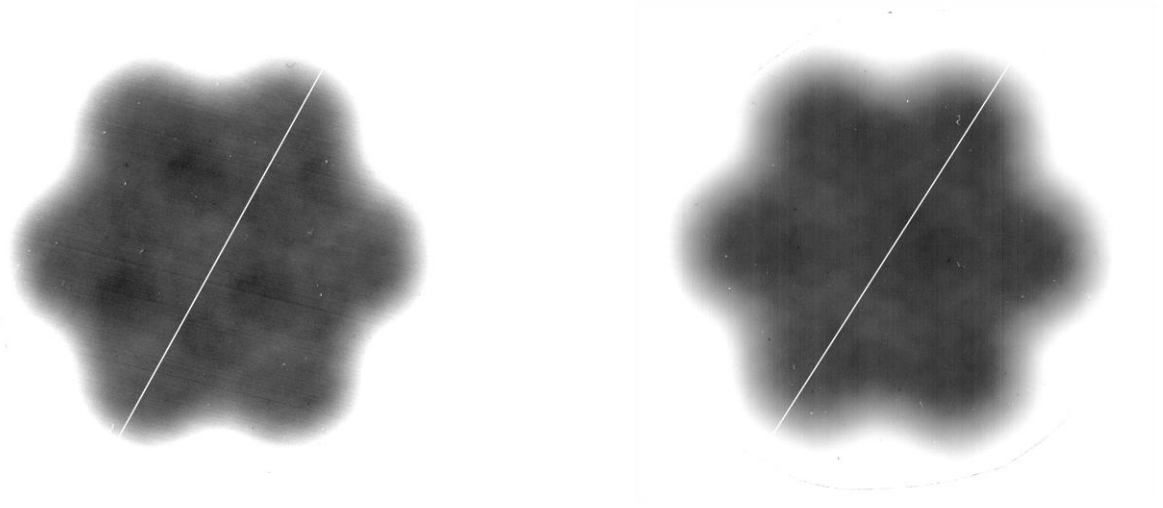
Figure 6: Optical density maps of Gafchromic ™ HD-V2 film irradiated using the 1800 \mu\text{m} (left) and 2600 \mu\text{m} (right) collimator, contrast enhanced to show the residual unevenness in dose distribution due to the honeycomb structure. Variations in dose distribution were below 5% for both collimators. The white lines are 30 mm long and indicate the position of the intensity profile in Figure 7. White specks are dust particles on the film during scanning.
