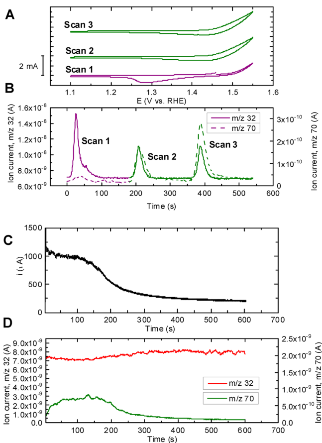
Figure 7. OLEMS measurements of an \text{IrO}_x/\text{GC} disk electrode in 0.5 M \text{KH}_2\text{SO}_4 , 80 mM \text{KCl} , and 1.2 mM \text{MnSO}_4 ( \text{pH} = 0.89 ). (A) CVs of the electrode after preconditioning for 450 s at 1.46 V, followed by three scans. Scan rate: 5 \text{ mV s}^{-1} . (C) Amperometry at 1.500 V for 600 s. (B and D) Corresponding OLEMS mass signals over time. Solution is saturated with Ar. A stirrer bar at \sim 600 \text{ rpm} was employed to increase mass transport.
