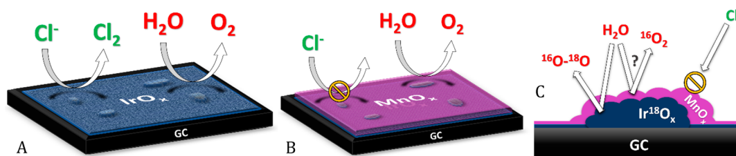
Scheme 1. Sketch of the IrO x /GC Catalyst (A), Deposition Structure of MnO x Deposition on MnO x /IrO x /GC (B), a and a Side-View (C) Showing the Isotopic Labeling Experiment in Figure 11A and B b
