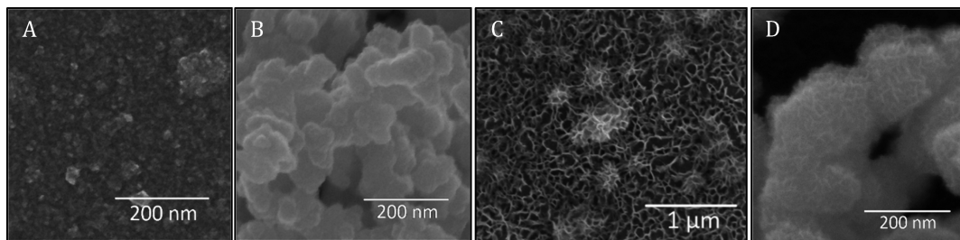
Figure 8. SEM micrographs of representative electrodes used in this study. (A and B) \text{IrO}_x/\text{GC} electrode, deposited according to the procedure described by Nakagawa et al. (C and D) \text{MnO}_x/\text{IrO}_x/\text{GC} electrode; \text{MnO}_x was deposited onto \text{IrO}_x/\text{GC} as described in the text.
