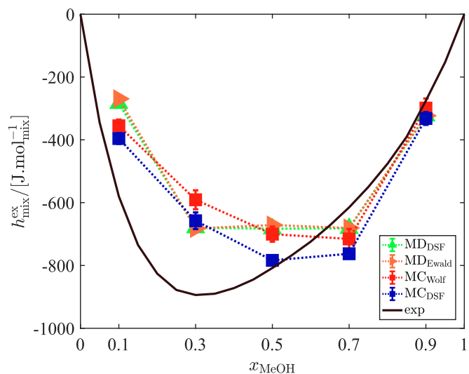
Figure 4. (Colour online) Excess enthalpies of mixing for water–methanol mixtures based on the TIP4P/2005 [17] and TraPPE [83] force fields at T=298 K and P=1 bar. To compute the electrostatic energies, the DSF and Ewald [92] methods were used in MD simulations. In MC simulations, the Wolf and DSF methods (Equations (3) and (5)) were used to treat the electrostatic interactions. The solid line indicates experimental values for the excess mixing enthalpy [49]. Dotted lines are a guide to the eye. Error bars are smaller than symbol sizes. Raw data are listed in Tables S1, S5 and S15 of the Supporting Information.
