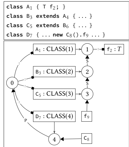
Fig. 9. Classes with inheritance. The P edges from scopes #1, #2, #3 to scope #0 have been omitted.
