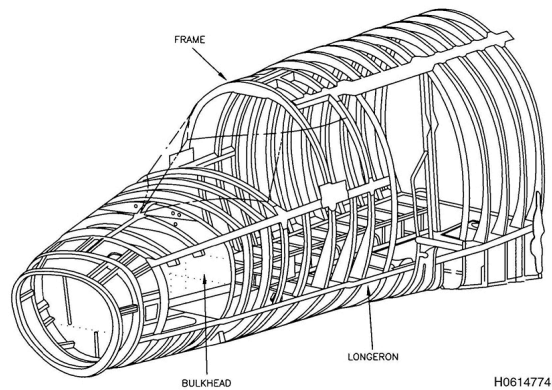
Figure 5.17 Longitudinal stiffness created with longerons. (Anon., n.d., Public Domain)
