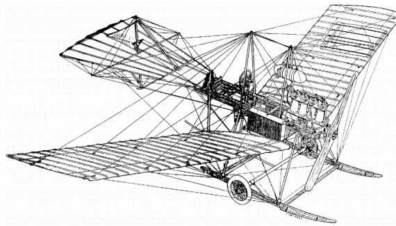
Figure 5.1 Illustration of the Fokker Spin or Fokker Spider. (Anon., n.d., 5-1.jpg. Public Domain.)
