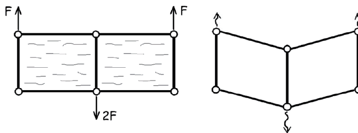
Figure 7.13 Elementary spar constructed from rigid girders and sheets (left) will deform if sheets are removed (right). . (TU Delft, n.d., 7-13.jpg. Own Work.)
