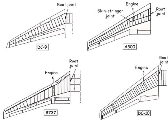
Figure 5.18 Comparison of four wing structural lay-outs. (TU Delft, n.d., 5-18.jpg. Own Work.)
