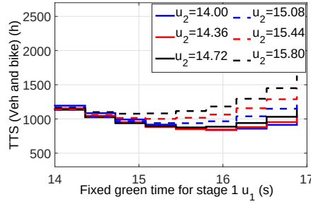
Figure 7: TTS as function of a fixed green time of the stage 1 u_1 and 6 cases for the stage 2 u_2 .
