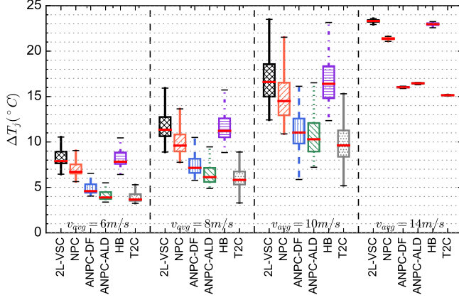
Figure 4.20 Distribution of temperature cycling amplitudes for the generator side converter.
