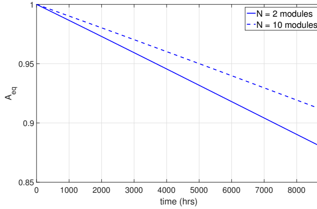
Figure 6.11 The effective availability of the converter system with time over one maintenance period T_m . An increase in the number of modules leads to a greater effective availability.
