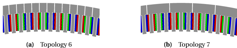
Figure 6.6 Segmentation with flux gaps in the stator yoke.
