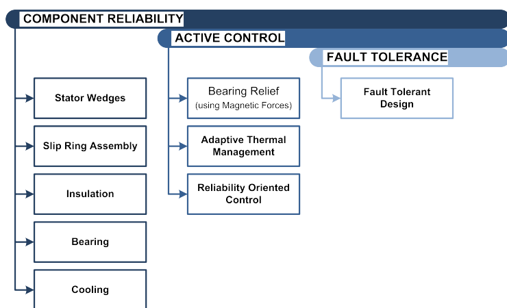
Figure 3.12 Framework for increasing generator availability.
