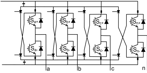
Figure 3.9 Double switch redundant topology.
