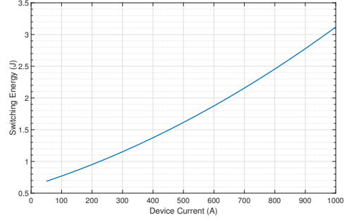
Figure 4.10 IGBT characteristics - E_{sw}
