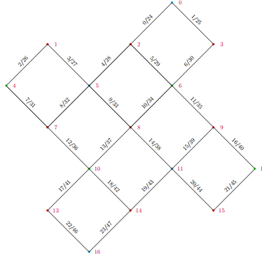
Figure 6.1: Quantum chip topology of the target 17-qubit superconducting quantum processor.
