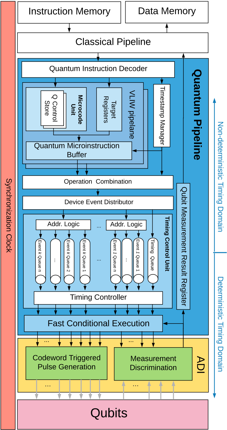
Figure 4.9: Quantum microarchitecture implementing the instantiated eQASM for the seven-qubit superconducting quantum processor.
