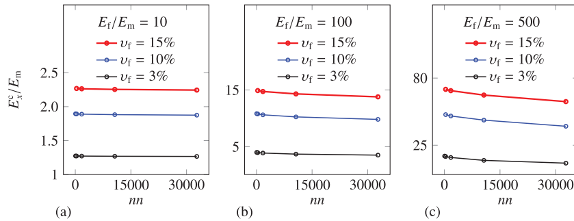
Fig. 17. Effective Young's modulus along the x-axis for a transversely isotropic composite with aligned fibers for different mesh densities ( nn indicates the number of mesh nodes) and fiber volume fractions \nu_f . In the calculations reported in Section 5 ( d_f = 0.007L and l_f = 0.2L ), the finest discretization with 31 \times 31 \times 31 trilinear hexahedral elements and 32768 nodes has been used.
