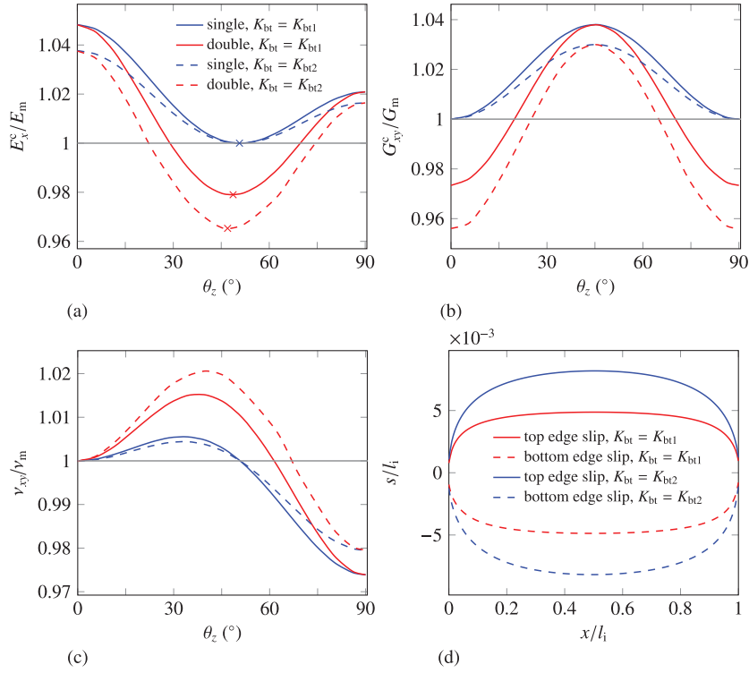
Fig. 15. Effective (a) Young's modulus, (b) shear modulus and (c) Poisson's ratios of a two-dimensional composite with imperfect interface ( K_{bt1} = 1000 N/mm 2 , K_{bt2} = 500 N/mm 2 , E_f/E_m = 10 and \nu_m = 0.4 in plane strain). The single-interface model shows neutrality for \theta = \theta_n ( \theta_n \approx 50.7^\circ from Fig. 7b), while the double-interface model predicts degraded effective mechanical properties compared with intact matrix properties. (d) Fiber interfacial slips for \theta = \theta_n using the double-interface model. (For interpretation of the references to colour in this figure legend, the reader is referred to the web version of this article.)
