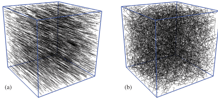
Fig. 16. Two realizations of a composite with approximately 4700 fiber (length l_f = 0.2L and diameter d_f = 0.007L ) in an L \times L \times L ( L = 1 mm) periodic simulation box resulting in a fiber volume fraction \nu_f = 3\% : (a) aligned and (b) randomly distributed fibers.
