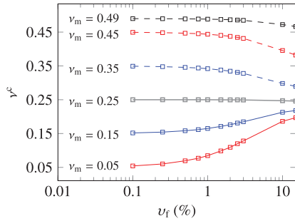
Fig. 21. Effective Poisson's ratios \nu^c of a nearly isotropic composite with randomly distributed fibers for different volume fractions \nu_f (matrix Poisson's ratios \nu_m , E_f/E_m = 100 , d_f = 0.007L and l_f = 0.2L ).
