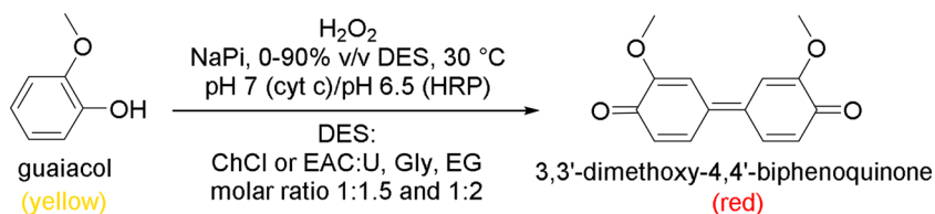
Fig. 14. Peroxidase activity assay for HRP and cyt c, determined by the colour change at 470 nm of guaiacol (yellow) to 3,3'-dimethoxy-4,4'-biphenylquinone (red) through oxidation by hydrogen peroxide (For interpretation of the references to colour in this figure legend, the reader is referred to the web version of this article).
