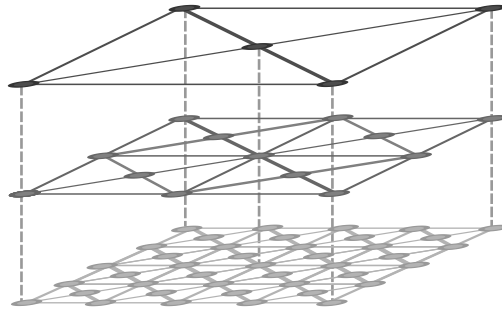
Figure 2.3: Isometric view of an example Tubes topology, which constrains traffic along all four dimensions of motion. The dashed lines are used to indicate the placement of nodes above each other.
