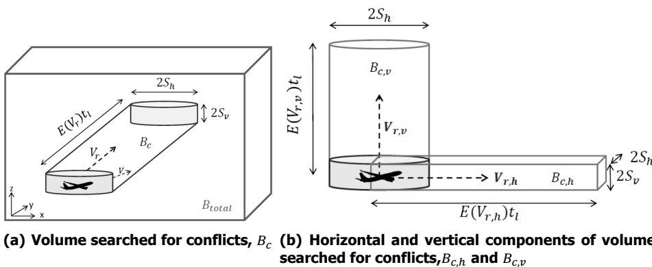
Figure 4.4: Volume searched for conflicts by an aircraft, B_c . Here, B_{total} is the total volume of the airspace. Note that B_c = B_{c,h} + B_{c,v}
