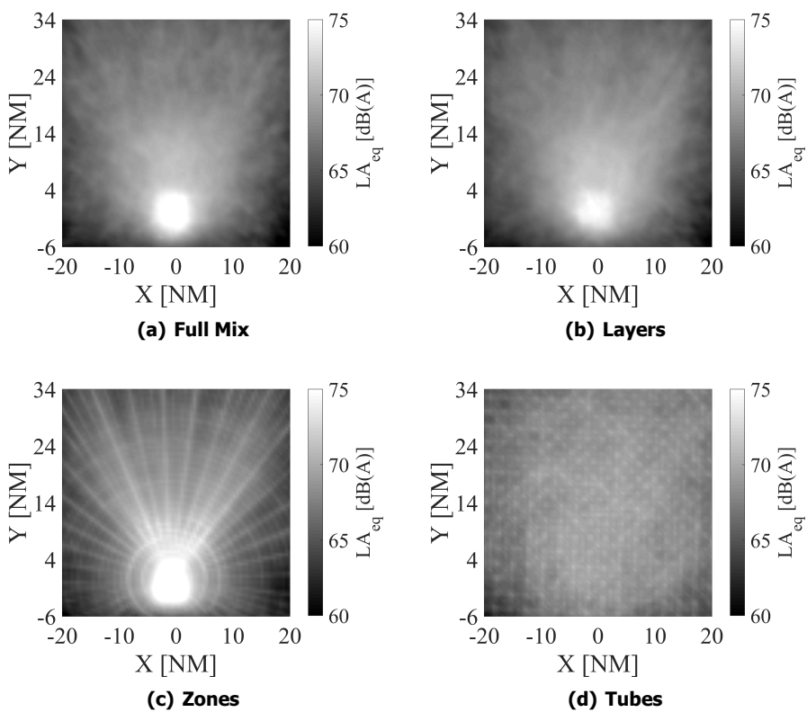
Figure 2.18: Noise footprints for an 'Ultimate' demand scenario with a converging traffic demand pattern
