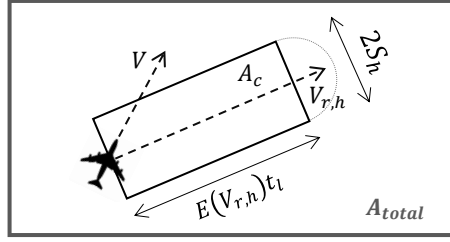
Figure 5.7: Area searched for conflicts, A_c , by cruising traffic in layered airspaces. Here, A_{total} is the total airspace area of one flight level.
