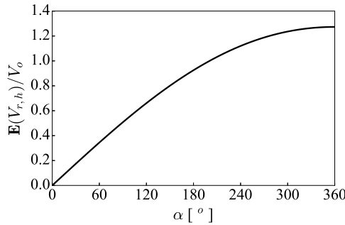
Figure 3.8: Hypothesized relationship between the expected horizontal relative velocity, E(V_{r,h}) , and heading range per flight level, \alpha
