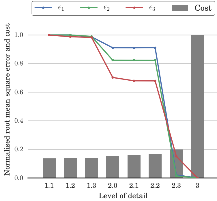
Figure 5: Errors and computation cost for each LOD. The metrics are normalised according to the least favourable result.
