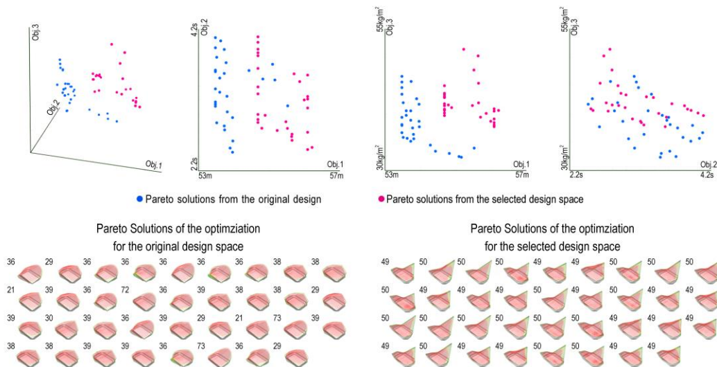
Figure 3: Results of the MOOs for the original design space and the selected design space (the cluster index of each solution is labeled beside it)
