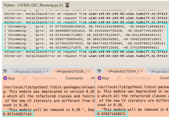
Figure 2: Top: OSC-data receiving and parsing. Bottom: 95.7% prediction success with respect to HAR via SVM (left) vs. 97.85% via k -NN (right).
