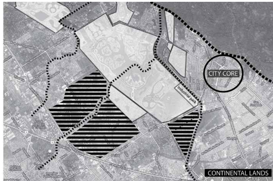
FIGURE 4.42 Floods in the continental area of Tigre due to the changes in topography and the blocking of water courses (Zagare, 2014a).
