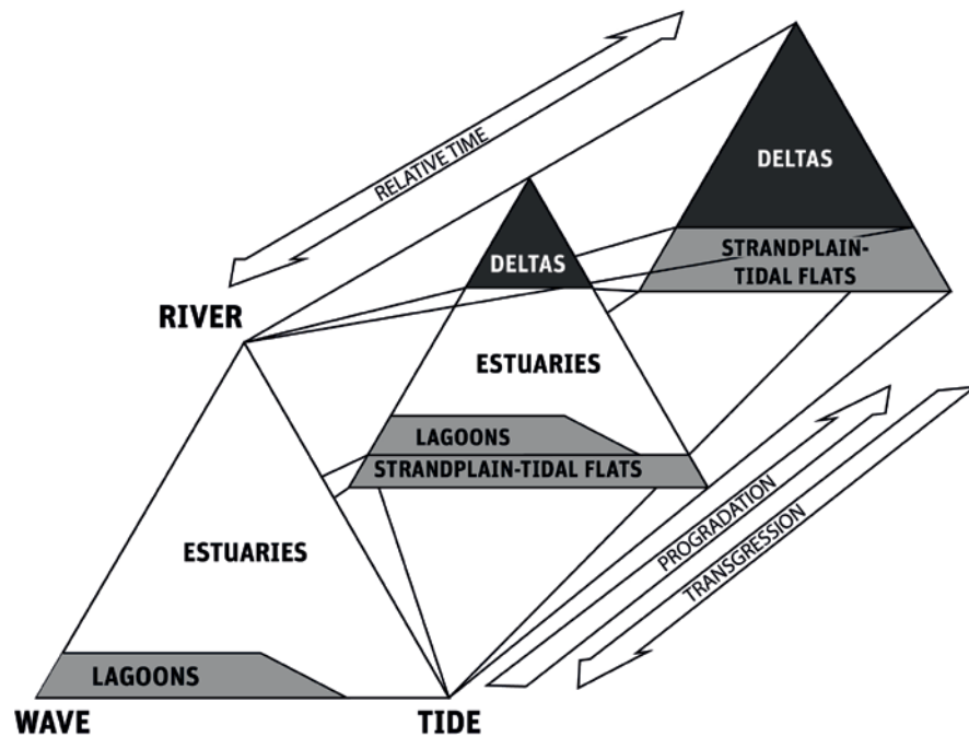
FIGURE 2.6 Evolution of the ternary diagram developed by Boyd et al. (1992, 144) according to the inclusion of prograding and transgressive processes.
