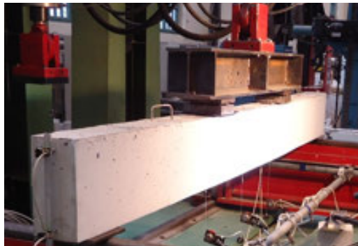
FIG. 12 Beam test
