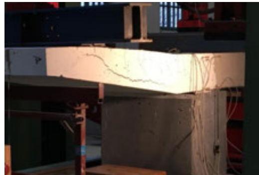
FIG. 13 Balcony test
