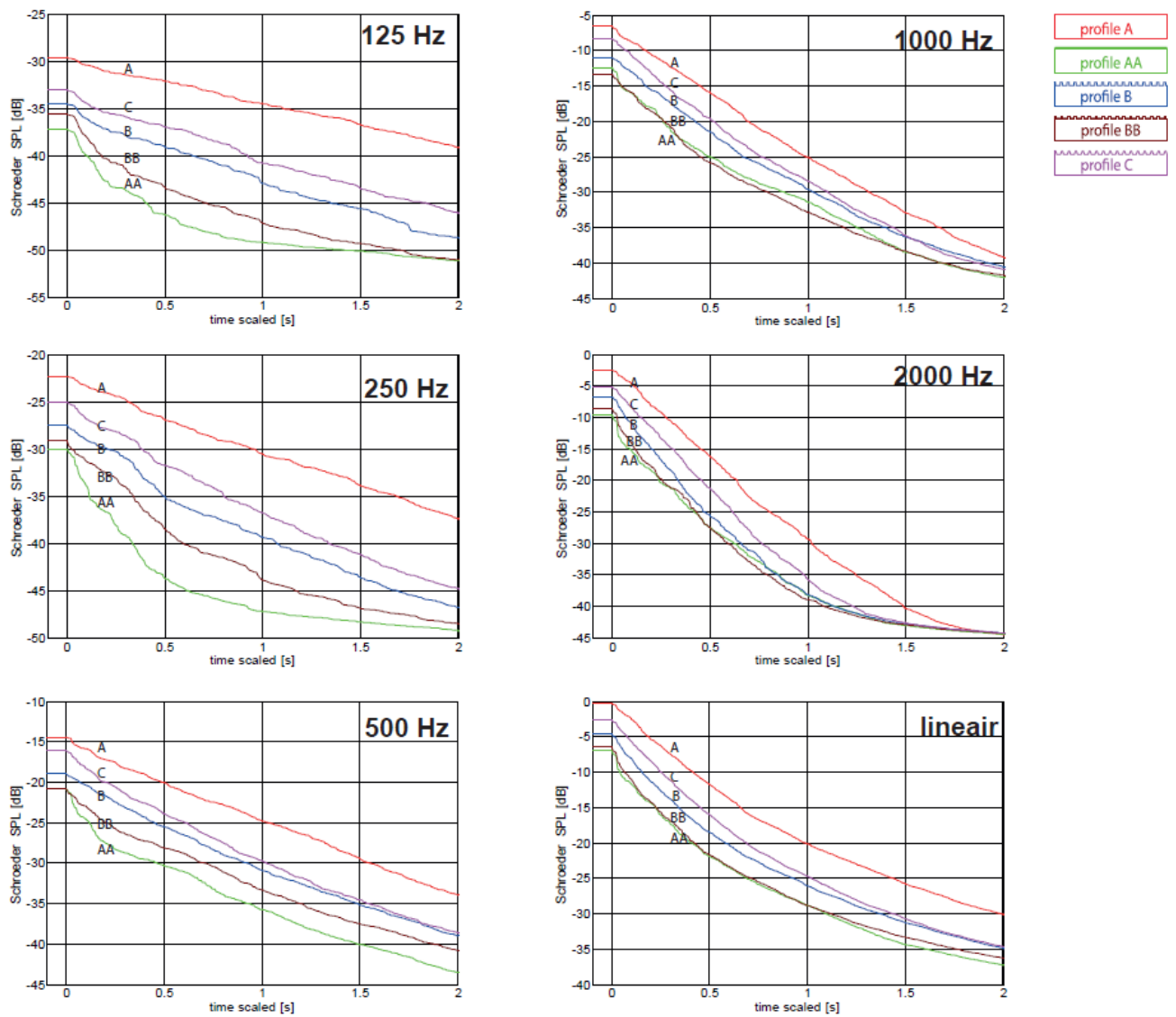
Figure 21 – Schroeeder curves of ‘closed box’ measurements on profiled roof structures with (AA, BB) and without absorption (A, B, C). Results per octave frequency band.
