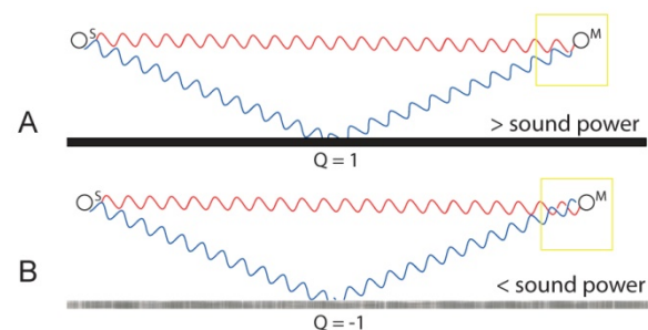
Figure 6 – Increase or decrease of sound power caused by interference.
