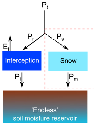
Figure 2. Schematisation of the method to calculate S_r , including snow module; the part in the red square is added for this research, the “endless” soil moisture reservoir is similar to the one in de Boer-Euser et al. (2016). The arrow for P_s is dashed as this flux is not actually calculated, but P_m is derived from the change in S_{SWE} .
