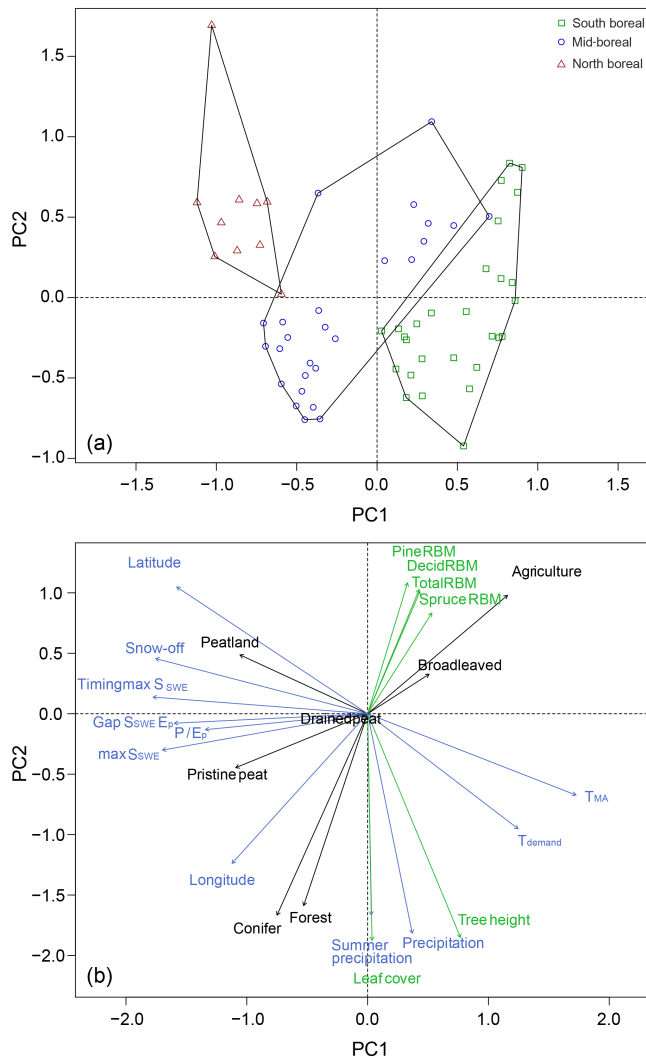
Figure 8. Principal component analysis with the catchment characteristics that are being compared with S_r in the study. (a) Catchments plotted on PC1 and PC2, with boreal regions indicated. (b) Catchment characteristics with their loadings on PC1 and PC2; catchment characteristics are divided into three categories: climate (blue), vegetation characteristics (green) and land use types (black). Note that for readability the axis of the two plots are not the same.
