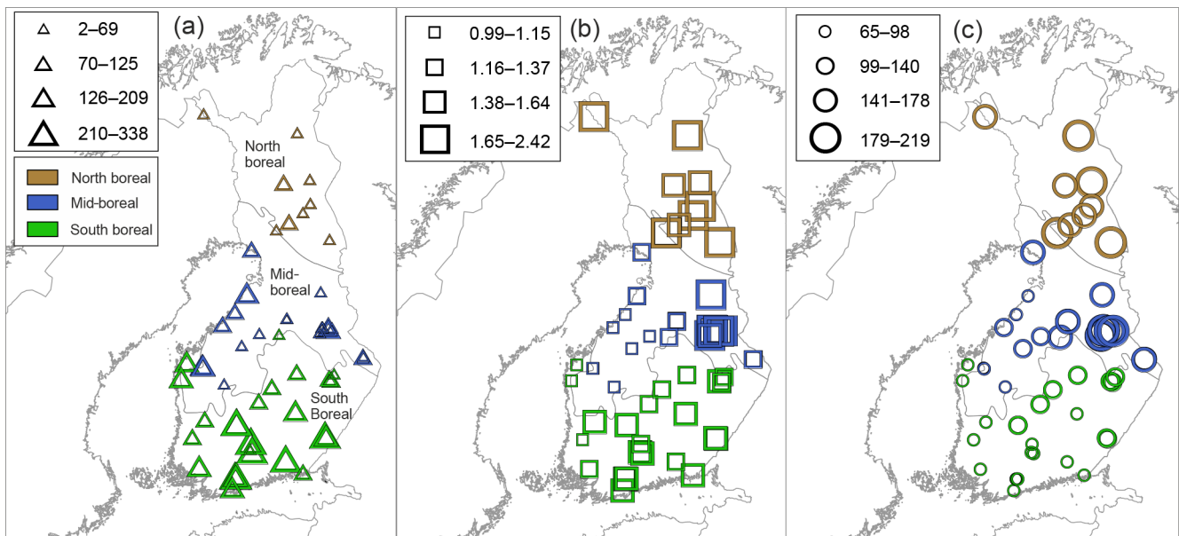
Figure 3. Map with study catchments and (a) calculated root zone storage values ( S_r , mm), (b) ratio of precipitation and potential evaporation, and (c) maximum snow water equivalent ( S_{SWE} , mm). Different boreal ecoregions (south boreal, mid-boreal and north boreal) are shown in the colours of the symbols and boundaries of ecoregions are marked with grey lines.
