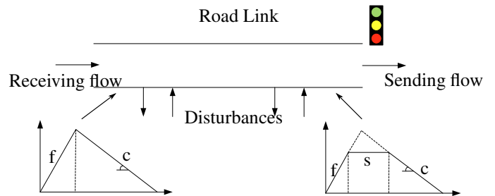
Figure 2. Signalized urban road link with upstream and downstream FDs
