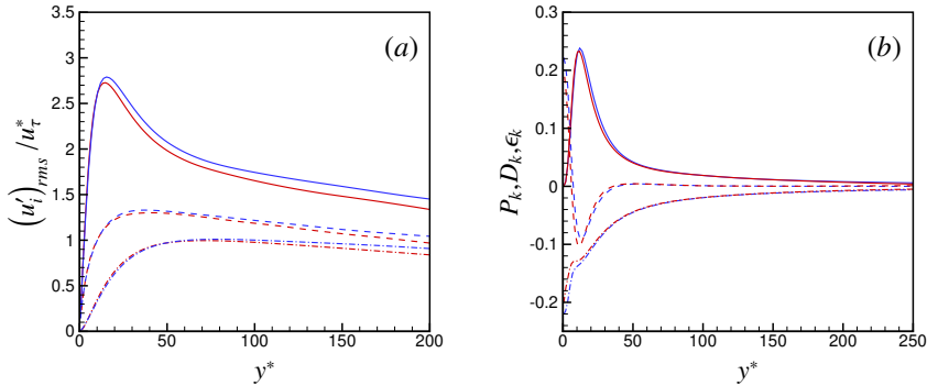
Figure 4.15: Semi-locally scaled velocity fluctuations and turbulent kinetic energy budgets as a function of y^* for LSC 2 . (a) (—) u'_{rms}/u_\tau^* ; (---) v'_{rms}/u_\tau^* (---) w'_{rms}/u_\tau^* . (b) (—) P_k ; (---) D_k ; (---) \epsilon_k . (—) Cold Side; (—) Hot Side.
