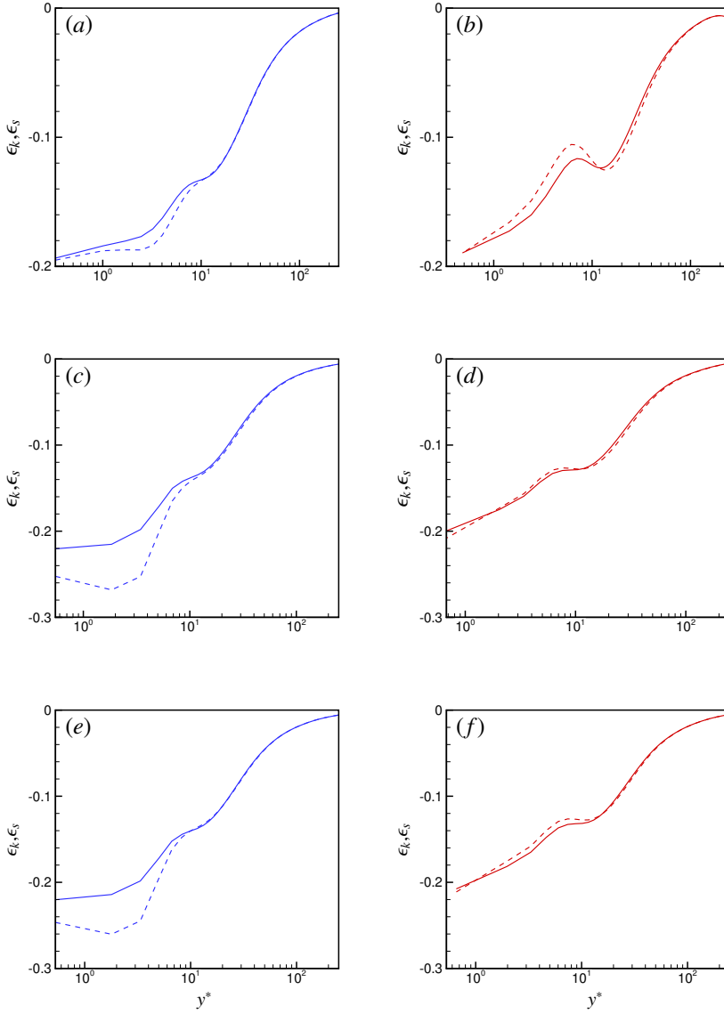
Figure 4.18: Solenoidal and total dissipation as a function of y^* for turbulent flows of supercritical \text{CO}_2 (—) \epsilon_k ; (---) \epsilon_s ; (—) Cold Side; (—) Hot Side. Top row: \text{HSC}_1 ; Middle row: \text{LSC}_2 ; Bottom row: \text{HSC}_2 .
