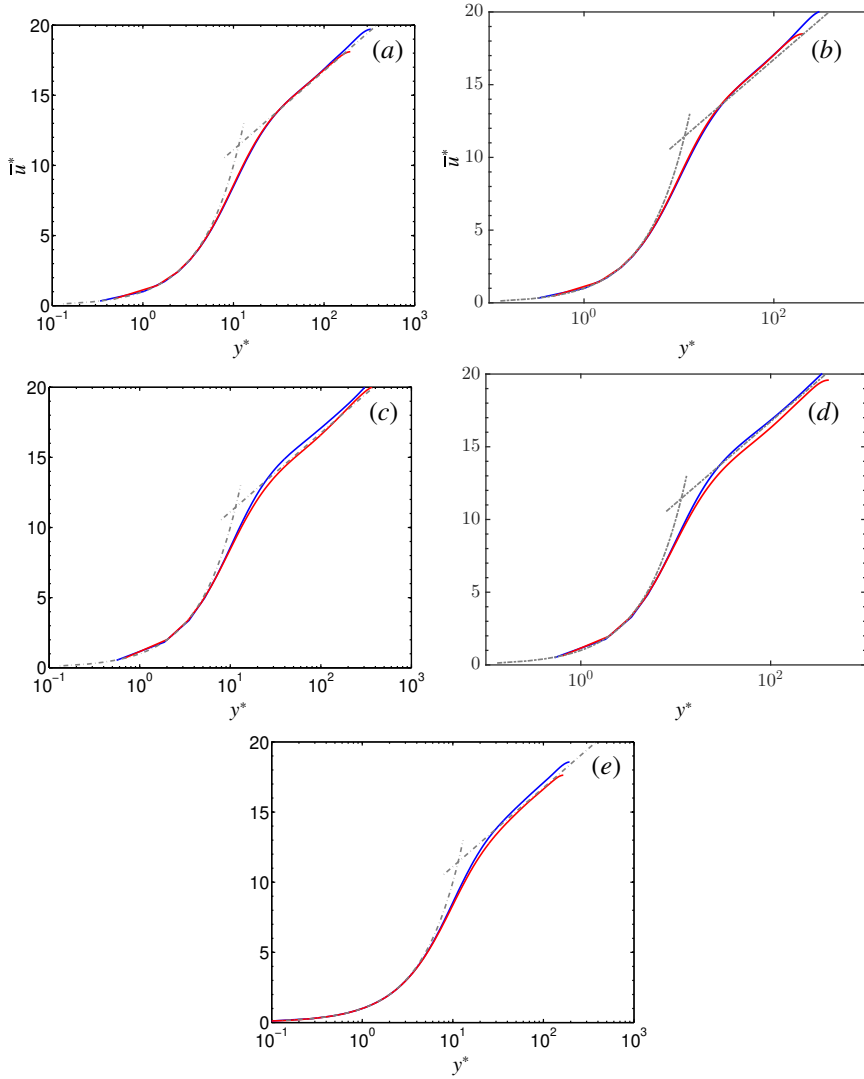
Figure 4.12: Extended van Driest transformed velocity as a function of y^* for turbulent flows of supercritical CO 2 . (a) LSC 1 ; (b) HSC 1 ; (c) LSC 2 ; (d) HSC 2 ; (e) SCCTP.
