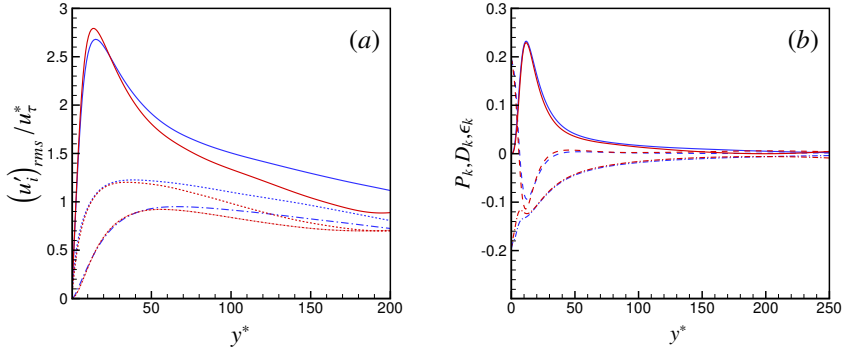
Figure 4.14: Semi-locally scaled velocity fluctuations and turbulent kinetic energy budgets as a function of y^* for HSC 1 . (a) (—) u'_{rms}/u_\tau^* ; (---) v'_{rms}/u_\tau^* (---) w'_{rms}/u_\tau^* . (b) (—) P_k ; (---) D_k ; (---) \epsilon_k . (—) Cold Side; (—) Hot Side.
