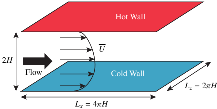
Figure 4.1: Flow geometry for fully developed turbulent channel flow with wall temperature difference
