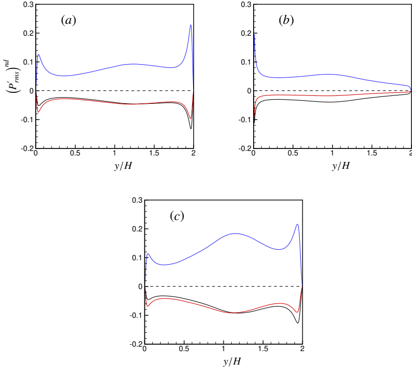
Figure 4.20: Contribution of the ideal, repulsive and the attractive components to the pressure fluctuations. (—) (P'_{rms})^{nd} (—) (P'_{rms})^{nd} (—) (P'_{rms})^{nd} ; (---) (P'_{rms})^{nd} ; (a) (LSC 1 ); (b) (LSC 2 ); (c) SCCTP.
