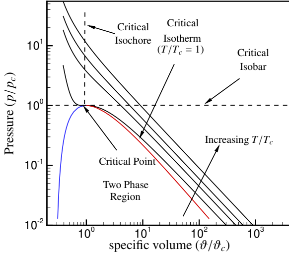
Figure 1.1: Pressure as a function of specific volume normalized by their critical values at constant temperatures for CO 2 ; (—) T/T_c = 1.0 ; T/T_c = 1.5 , T/T_c = 2.0 , T/T_c = 3.0 ; (—) Saturation liquid line; (—) Saturation vapour line.
