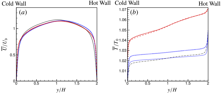
Figure 4.2: Mean velocity and mean temperature as a function of channel height for turbulent flows of supercritical \text{CO}_2 . (a) Mean velocity; (b) Mean temperature; (—) \text{LSC}_1 ; ( \blacktriangle ) \text{HSC}_1 ; (---) \text{LSC}_2 ; ( \blacktriangledown ) \text{HSC}_2 ; (---) \text{SCCTP} .
