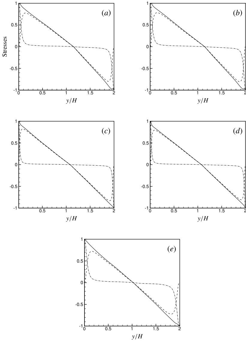
Figure 4.6: Shear stresses as a function of channel height for turbulent flows of supercritical CO 2 . (---) -\overline{\rho u'v'}/\tau_w ; (-.-) (\overline{\mu} \partial \overline{U} / \partial y) / \tau_w ; (—) (-\overline{\rho u'v'} + \overline{\mu} \partial \overline{U} / \partial y) / \tau_w . (a) LSC 1 ; (b) HSC 1 ; (c) LSC 2 ; (d) HSC 2 ; (e) SCCTP.
