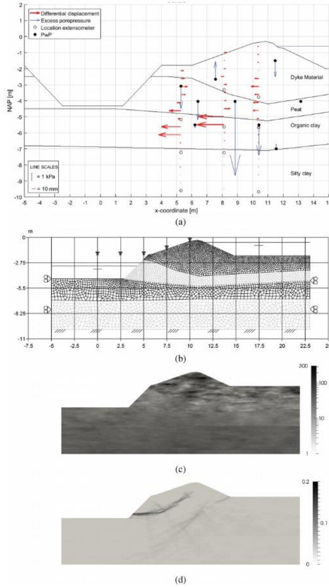
Figure 1. Analysis of the embankment: (a) measured differential displacements and excess pore pressures at the moment of failure; (b) finite element mesh used for analysis, with triangles indicating CPT locations, water level in ditch at NAP -3.15 m and waterlevel upstream at NAP -0.6 m; (c) example of an RFEM analysis, with shear strength illustrated on a logarithmic scale in kPa (d) the calculated shearbands as contours of deviatoric strain.
