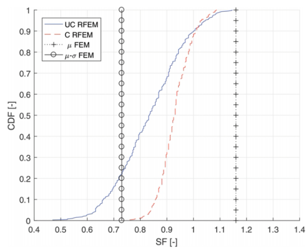
Figure 2. Analyses results for safety factor (SF).
