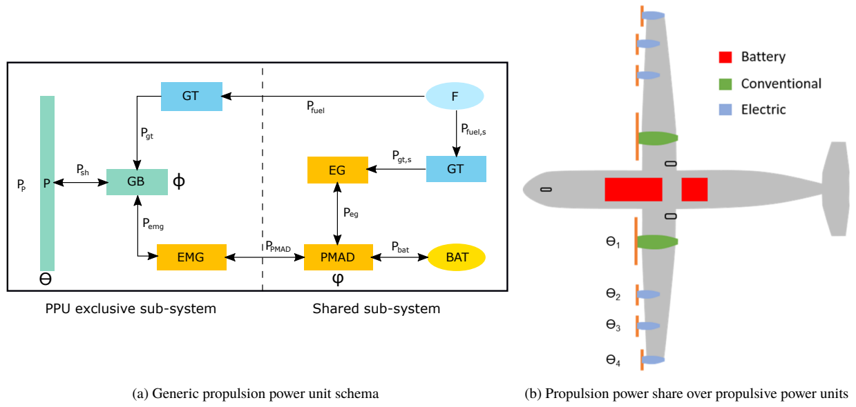
Fig. 2 Generalization of the propulsion power unit with main control parameters and power-paths
