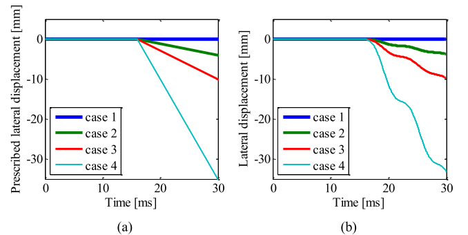
Fig. 3. Time histories of the prescribed displacement boundary conditions and the resulting lateral wheel displacements. (a) Prescribed displacement boundary conditions applied to the simulation cases; (b) simulated resulting lateral wheel displacements.
