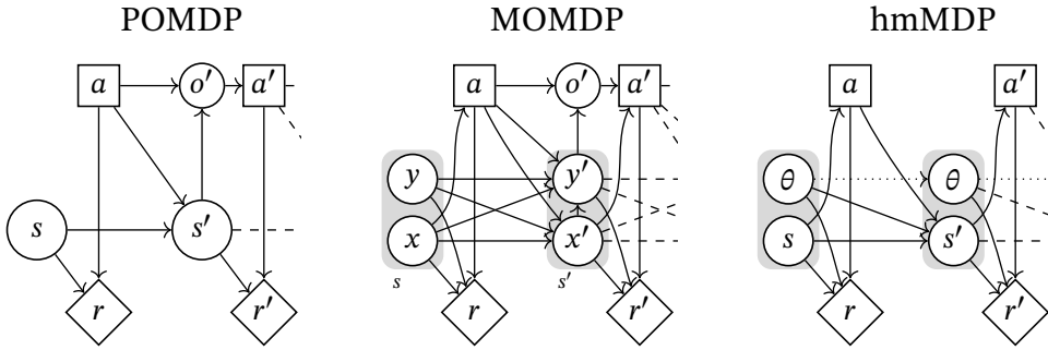
Figure 5.1: Comparison of the models of partial observability through their dynamic Bayesian networks (Boutillier, Dean, and Hanks, 1999). Nodes represent states and observations (circles), decisions (squares) and rewards (diamonds), while edges encode direct stochastic influences.
