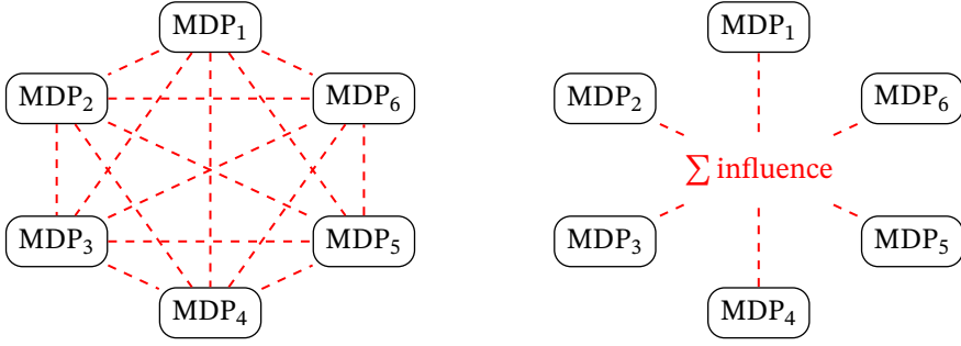
Figure 2.1: Constraints impose an all-to-all coupling between the otherwise independent single-agent MDPs ( left ). The weak coupling imposed by constraints suggests abstracting the influence agents have on each other ( right ).
