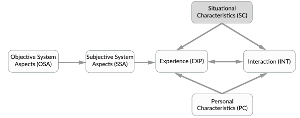
Figure 2: The user-centric evaluation framework of recommenders as used in our experiment, while our model does not contain situational characteristics (SC).
